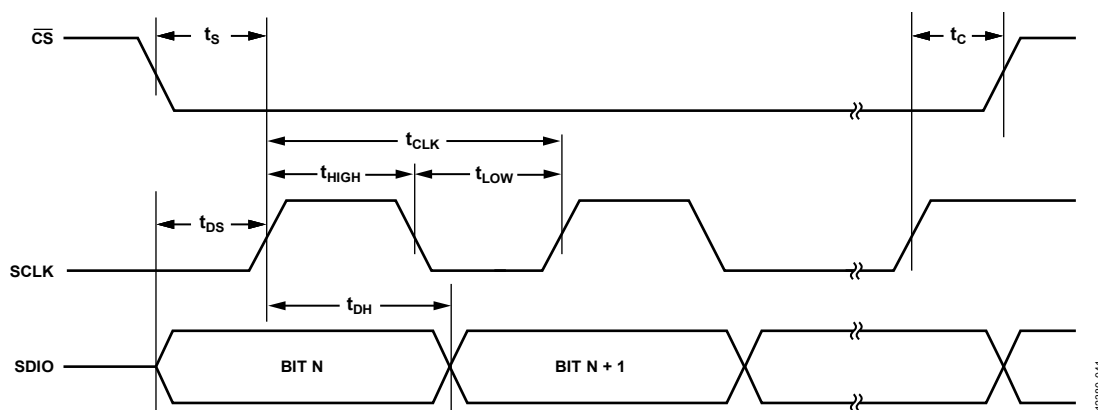
Figure 45. Serial Control Port Timing—Write
