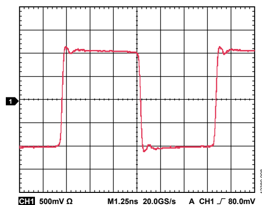
Figure 8. Output Waveform (Differential), HSTL at 122.88 MHz
