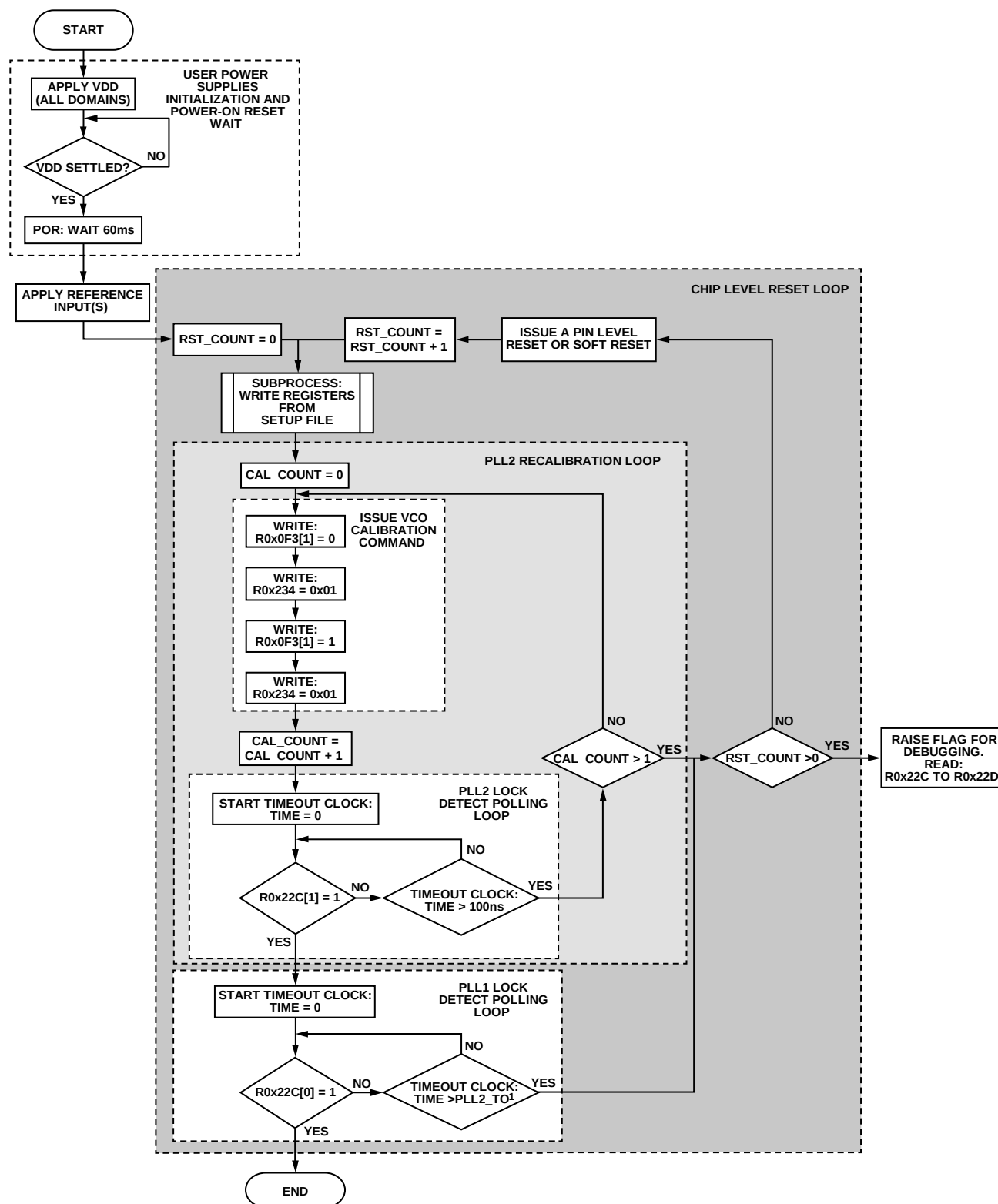
Figure 46. AD9523-1 Device Initialization
