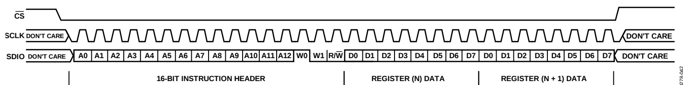
Figure 44. Serial Control Port Write—LSB First, 16-Bit Instruction, Two Bytes of Data
