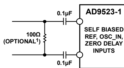
1 RESISTOR VALUE DEPENDS UPON REQUIRED TERMINATION OF SOURCE. Figure 23. REF, OSC_IN, and Zero Delay Input Differential Mode
