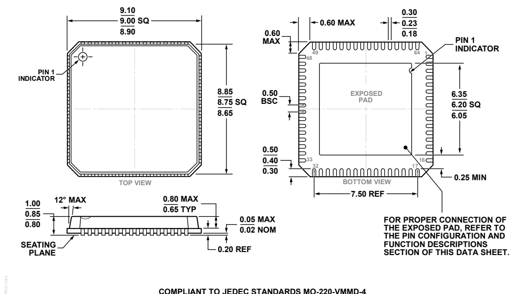
Figure 75. 64-Lead Lead Frame Chip Scale Package [LFCSP_VQ]
