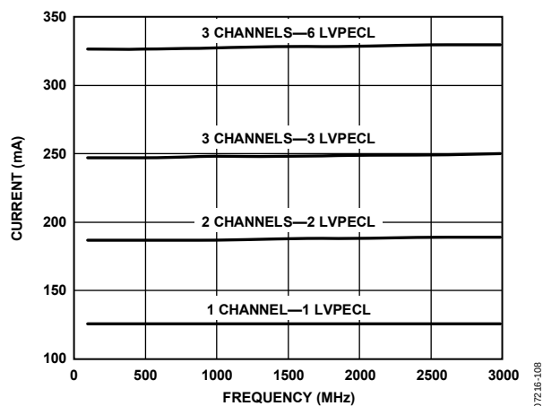
Figure 6. Total Current vs. Frequency, CLK-to-Output (PLL Off), LVPECL Outputs Terminated 50 \Omega to V_{S,DRV} = 2\text{ V}
