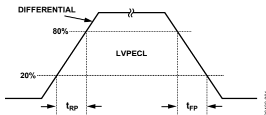
Figure 3. LVPECL Timing, Differential
