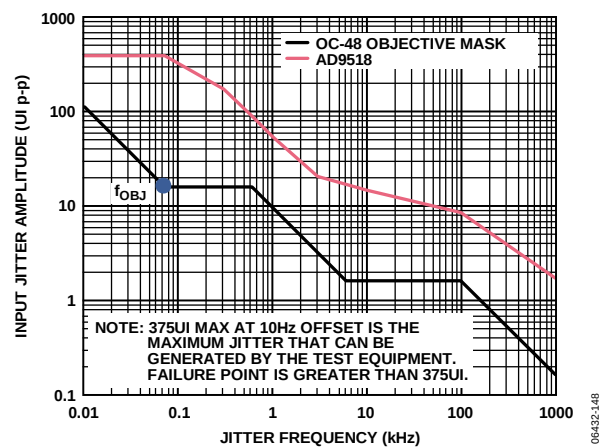
Figure 26. GR-253 Jitter Tolerance Plot
