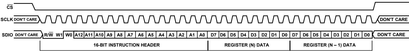
Figure 52. Serial Control Port Write—MSB First, 16-Bit Instruction, Two Bytes of Data
