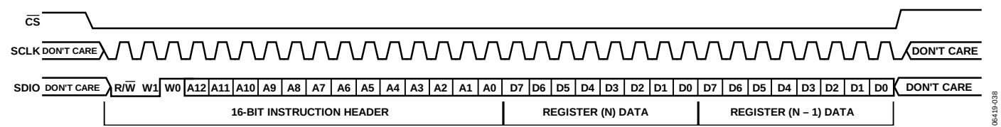
Figure 64. Serial Control Port Write—MSB First, 16-Bit Instruction, Two Bytes Data
