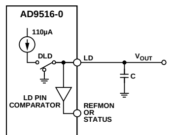
Figure 51. Current Source Lock Detect
