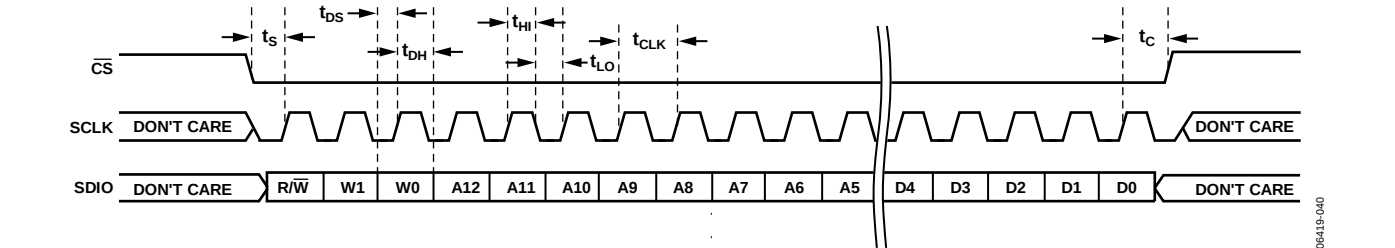
Figure 66. Serial Control Port Write—MSB First, 16-Bit Instruction, Timing Measurements
