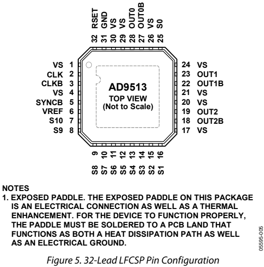
Figure 5. 32-Lead LFCSP Pin Configuration
