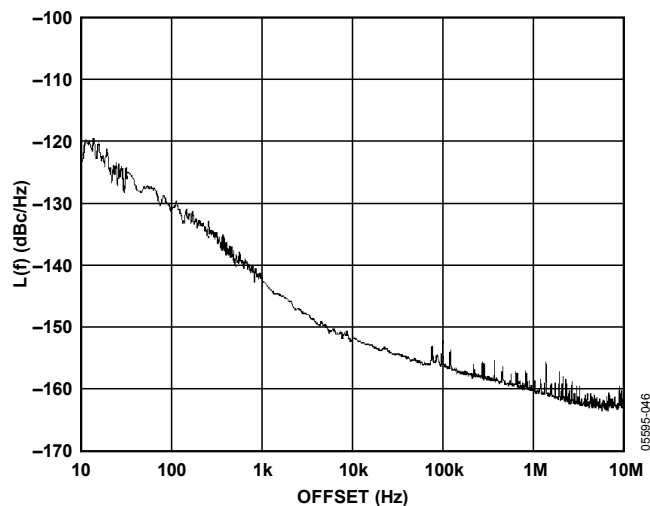
Figure 16. Additive Phase Noise—CMOS DIV4, 61.44 MHz
