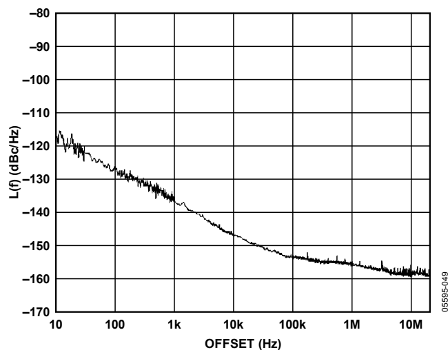
Figure 15. Additive Phase Noise—LVDS DIV2, 122.88 MHz
