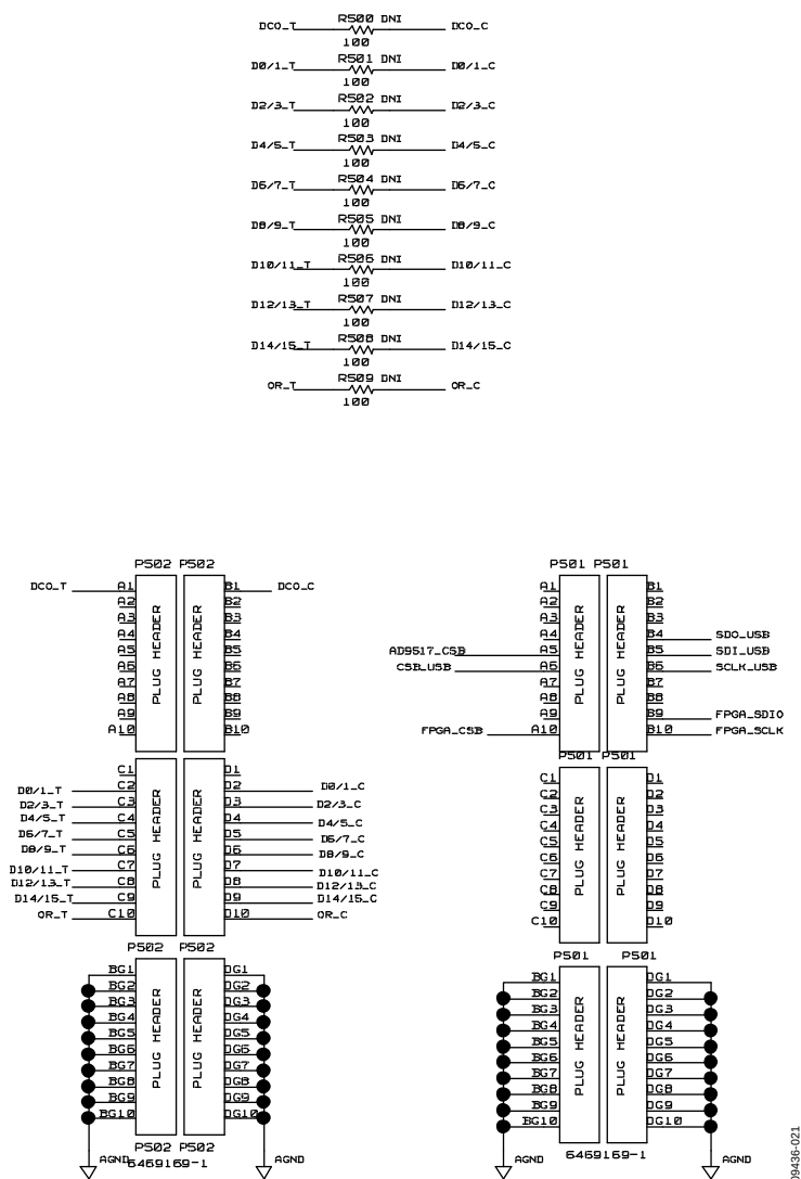
Figure 21. Digital Output Interface
