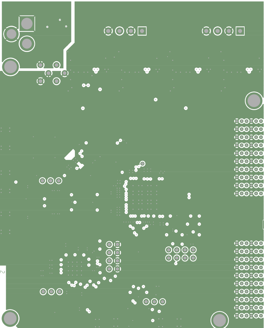
Figure 25. Ground (Layer 2)
