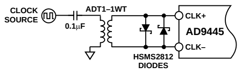
Figure 64. Crystal Clock Oscillator, Differential Encode
