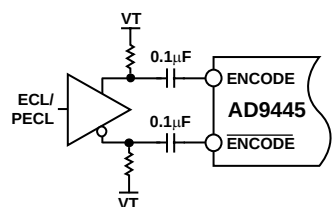
Figure 65. Differential ECL for Encode
