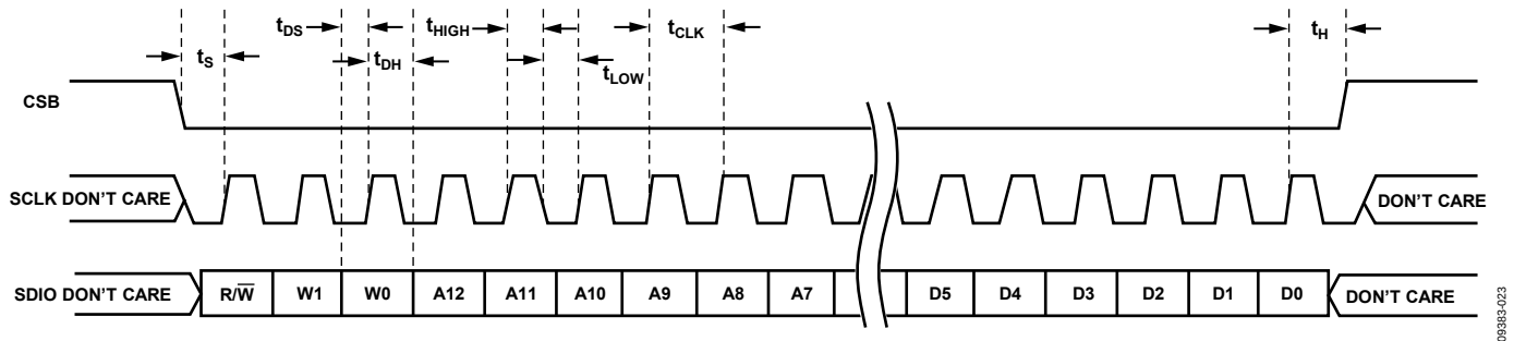
Figure 52. Serial Port Interface Timing Diagram
