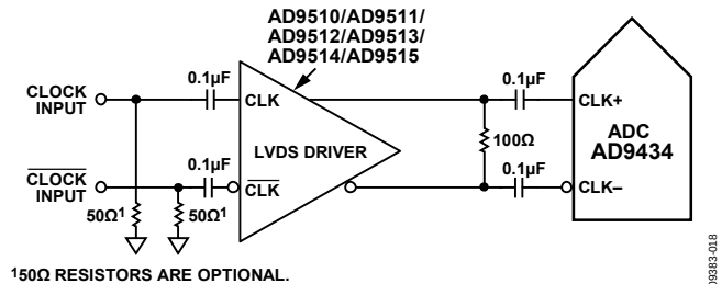
Figure 46. Differential LVDS Sample Clock
