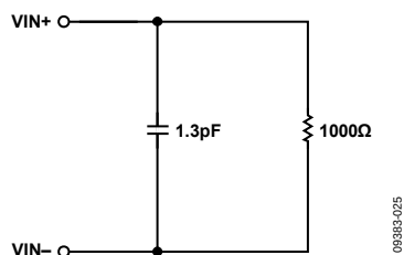
Figure 36. Analog Input AC Equivalent Circuit
