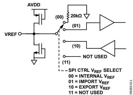
Figure 39. Equivalent VREF Input/Output Circuit
