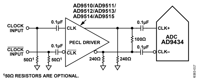
Figure 45. Differential PECL Sample Clock
