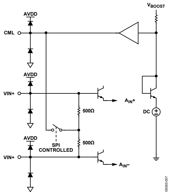
Figure 34. Analog Input DC Equivalent Circuit ( V_{CML} \approx 1.7V )
