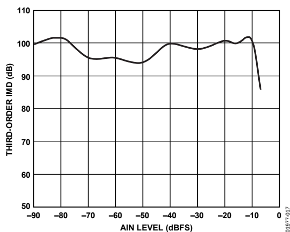
Figure 12. Third-Order IMD vs. AIN Level, f_s = 105 MSPS, f_{IN} = 49.3 MHz and 50.3 MHz, Differential AIN, SFDR Mode Enabled
