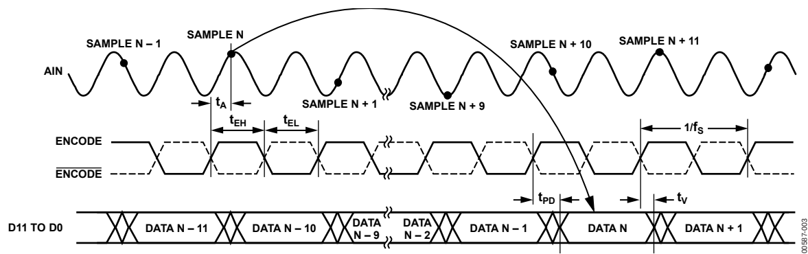
Figure 2. Timing Diagram
