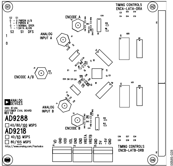
Figure 28. Top Silkscreen
