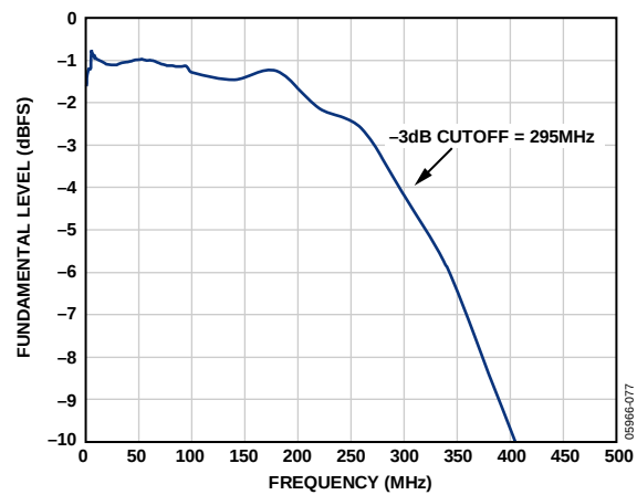
Figure 34. Full-Power Bandwidth vs. Frequency, f_{SAMPLE} = 100\text{ MSPS}
