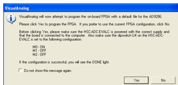
Figure 4. VisualAnalog Default Configuration Message
