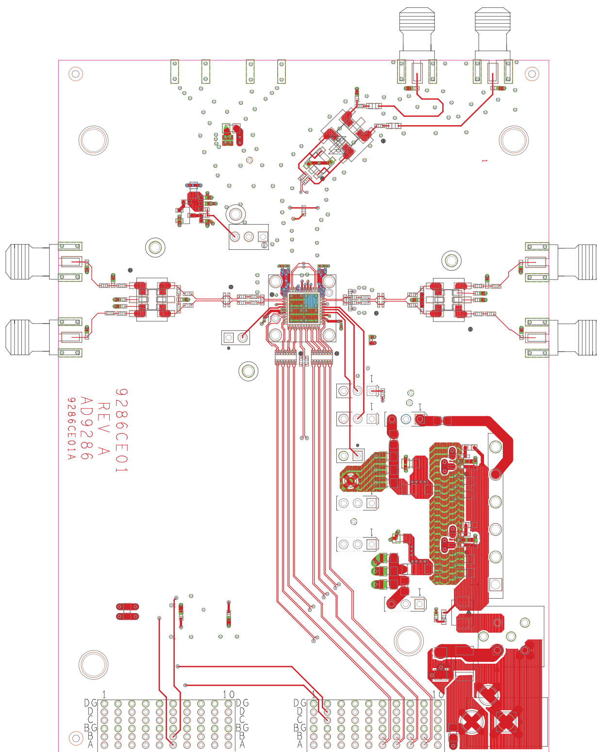
Figure 20. Top Side
