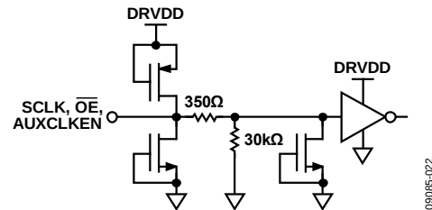
Figure 16. SCLK, \overline{OE}
