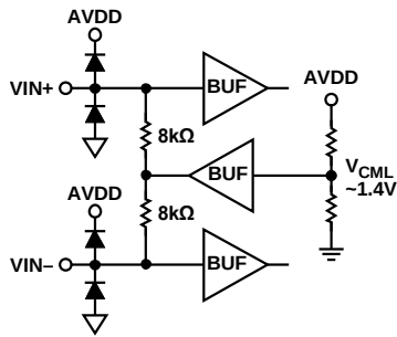
Figure 14. Analog Inputs ( V_{CML} \approx 1.4V )
