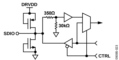
Figure 17. SDIO
