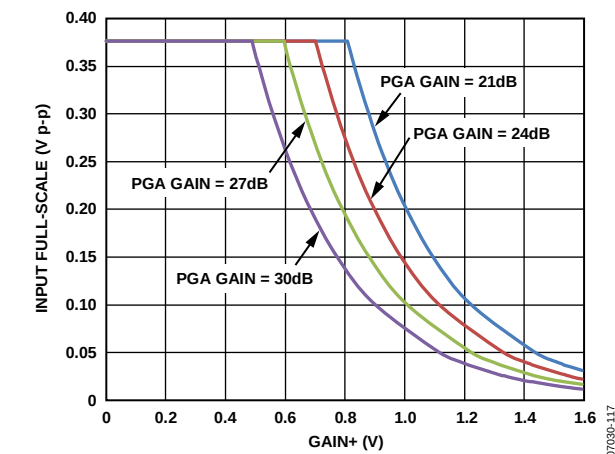
Figure 48. LNA with 15.6 dB Gain Setting/VGA Full-Scale Limitations
