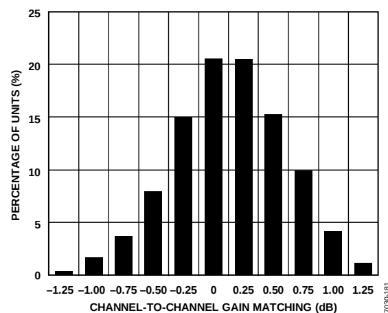
图11. 增益匹配直方图, GAIN+ = 1.3 V
