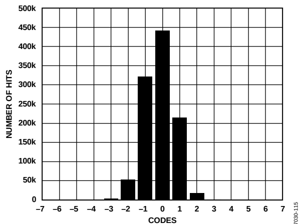
图12.折合到输出端的噪声柱状图, GAIN+ = 0.0\text{ V}
