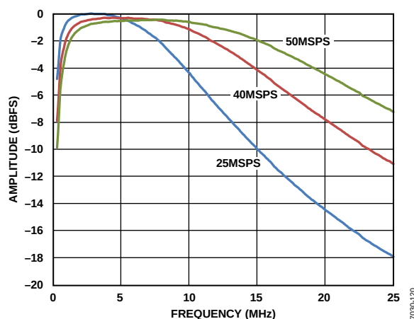
图17.抗混叠滤波器(AAF)通带响应, LPF 截止频率 = 1 \times (1/3) \times f_{SAMPLE}
