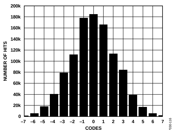
图13.折合到输出端的噪声柱状图, GAIN+ = 1.6\text{ V}
