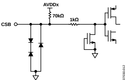
Figure 32. Equivalent CSB Input Circuit
