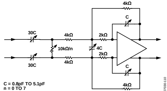
Figure 54. Simplified Filter Schematic
