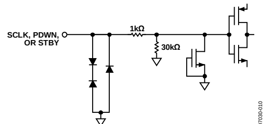
Figure 30. Equivalent SCLK, PDWN, or STBY Input Circuit
