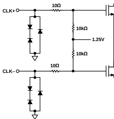
Figure 27. Equivalent Clock Input Circuit
