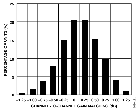
Figure 11. Gain Match Histogram, GAIN+ = 1.3 V
