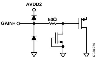
Figure 34. Equivalent GAIN+ Input Circuit
