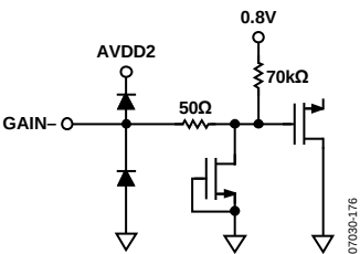
Figure 35. Equivalent GAIN- Input Circuit
