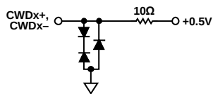
Figure 36. Equivalent CWDx± Output Circuit
