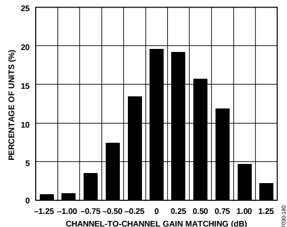
Figure 10. Gain Match Histogram, GAIN+ = 0.3 V
