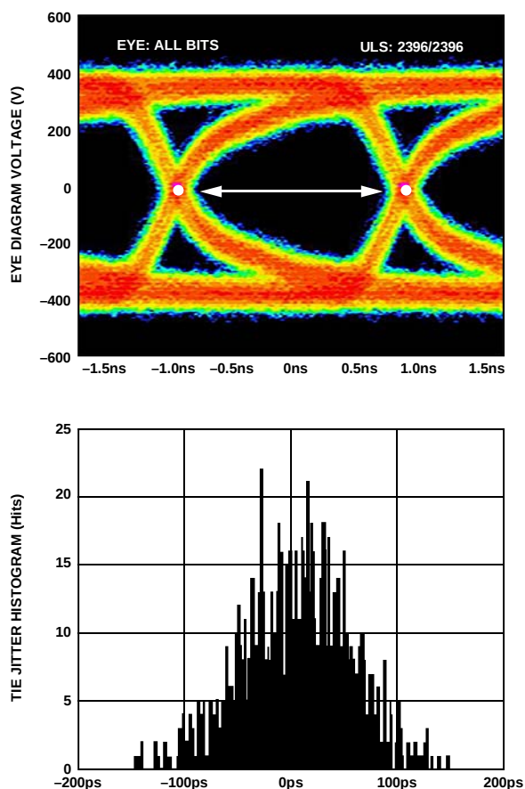
Figure 67. Data Eye for LVDS Outputs in ANSI-644 Mode with 100 \Omega Termination Resistor and Trace Lengths of Greater than 24 Inches on Standard FR-4
