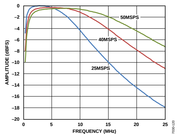
Figure 17. Antialiasing Filter (AAF) Pass-Band Response, LPF\text{ Cutoff} = 1 \times (1/3) \times f_{SAMPLE}
