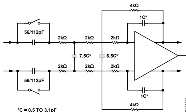
Figure 45. Simplified Filter Schematic
