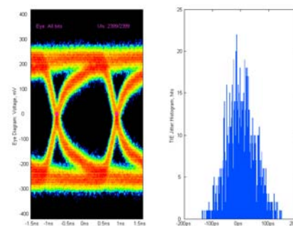
Figure 57. Data Eye for LVDS Outputs in ANSI Mode with 100 \Omega Termination on and Trace Lengths of Greater than 24 Inches on Standard FR-4
