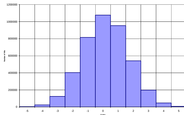
Figure 21. Output-Referred Noise Histogram with Gain Pin at 1.0V, AD9271-50
