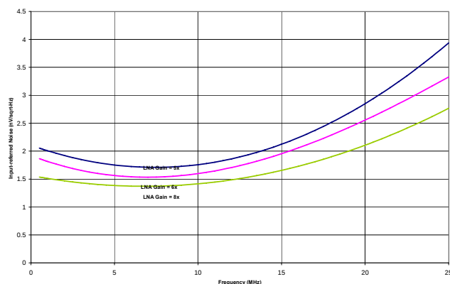
Figure 22. Short-Circuit, Input-Referred Noise vs. Frequency
