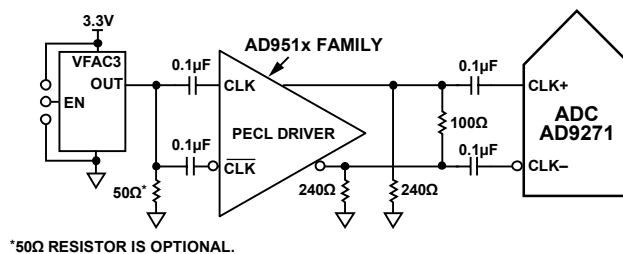
Figure 47. Differential PECL Sample Clock
