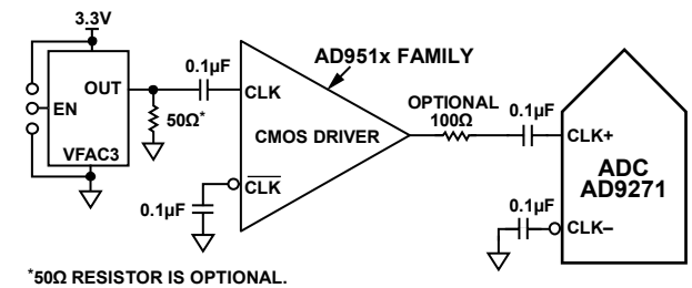
Figure 50. Single-Ended 3.3 V CMOS Sample Clock
