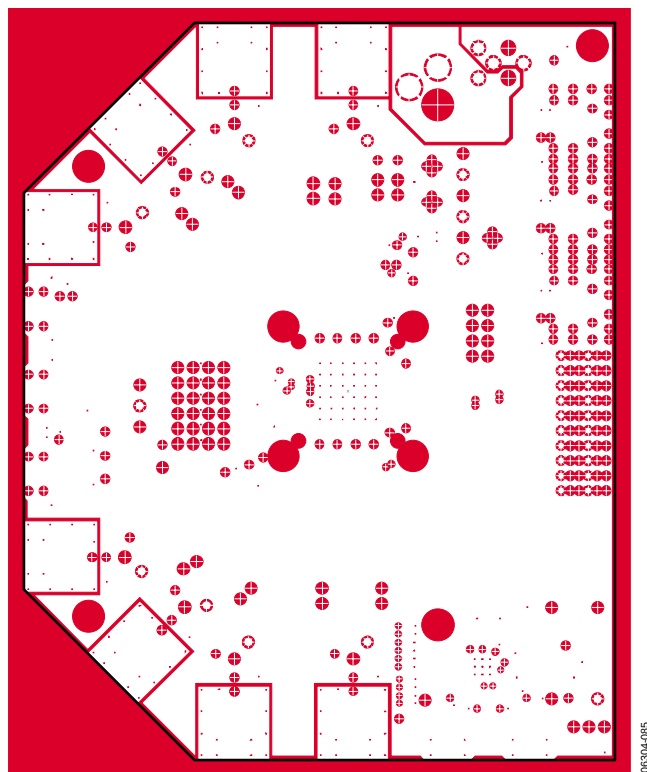
Figure 76. Evaluation Board Layout, Ground Plane (Layer 5)
