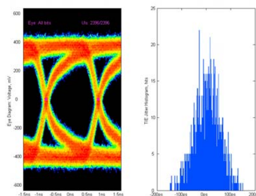
Figure 56. Data Eye for LVDS Outputs in ANSI Mode with Trace Lengths of Greater than 24 Inches on Standard FR-4
