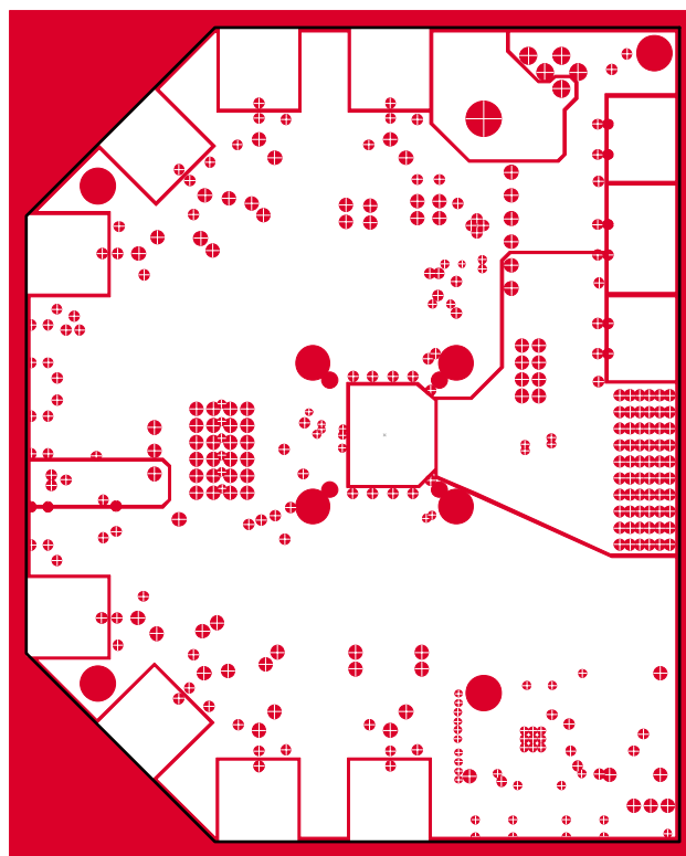
Figure 73. Evaluation Board Layout, Ground Plane (Layer 2)
