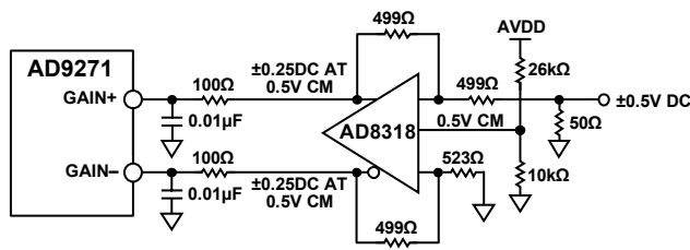
Figure 44. Differential Gain Pin Configuration
