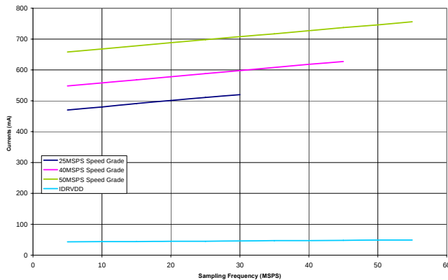
Figure 52. Supply Current vs. f_{\text{SAMPLE}} for f_{\text{IN}} = 7.5 \text{ MHz}
