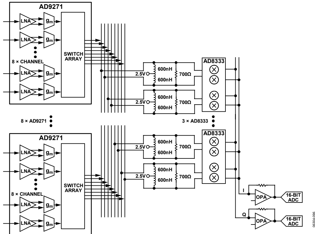
Figure 40. Typical CW Doppler System Using the AD9271 and AD8339
