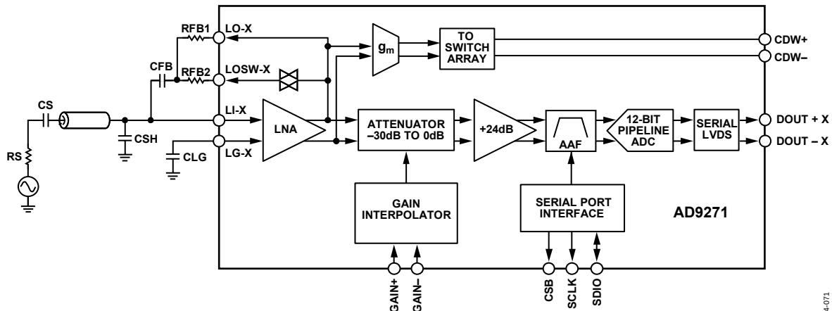
Figure 33. Simplified Block Diagram of Single Channel
