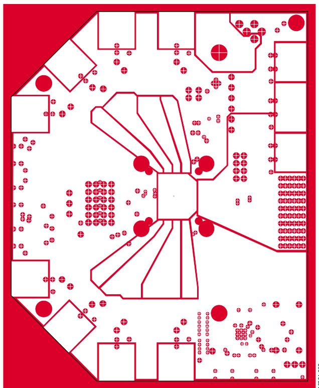
Figure 74. Evaluation Board Layout, Power Plane (Layer 3)
