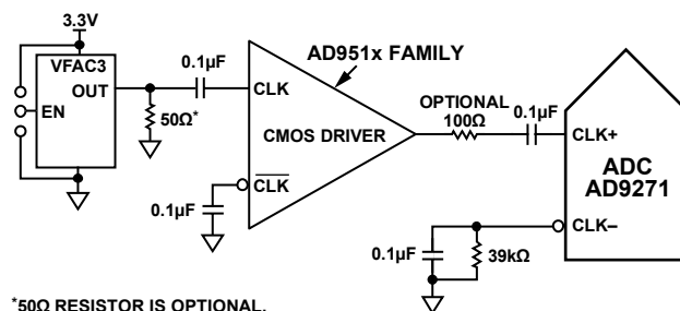
Figure 49. Single-Ended 1.8 V CMOS Sample Clock
