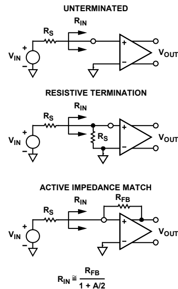
Figure 36. Input Configurations
