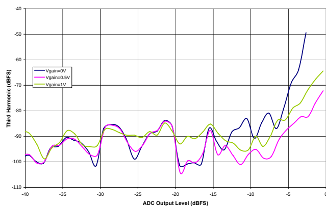
Figure 31. Third-Order Harmonic Distortion vs. ADC Output Level
