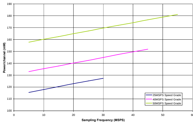
Figure 53. Power per Channel vs. f_{\text{SAMPLE}} for f_{\text{IN}} = 7.5 \text{ MHz}
