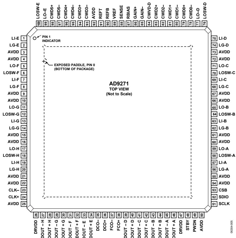
Figure 4. 100-Lead TQFP
