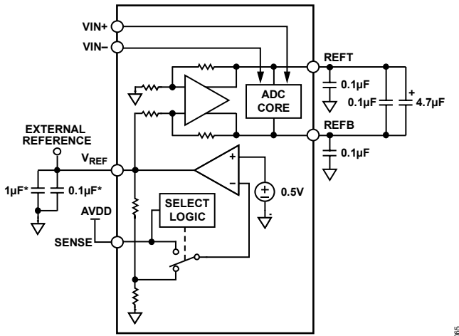
Figure 59. External Reference Operation
