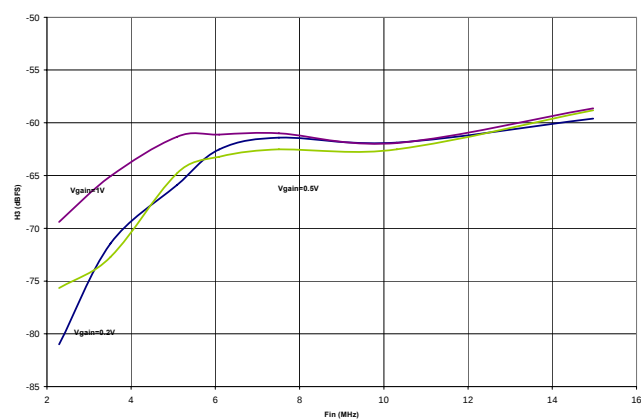
Figure 29. Third-Order Harmonic Distortion vs. Frequency
