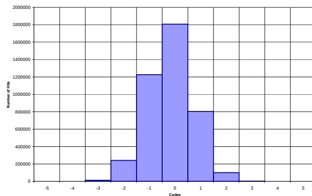
Figure 20. Output-Referred Noise Histogram with Gain Pin at 0.0V, AD9271-50
