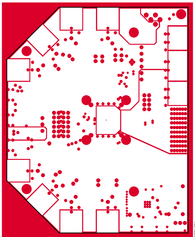
Figure 75. Evaluation Board Layout, Power Plane (Layer 4)
