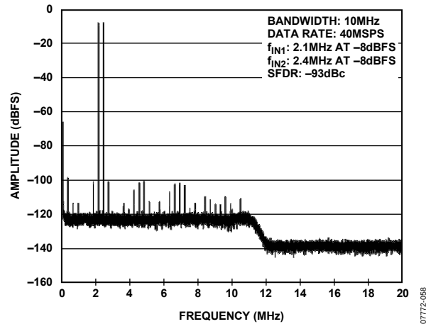
Figure 19. AD9262BCPZ-10 Two-Tone FFT with f_{IN1} = 2.1 MHz, f_{IN2} = 2.4 MHz
