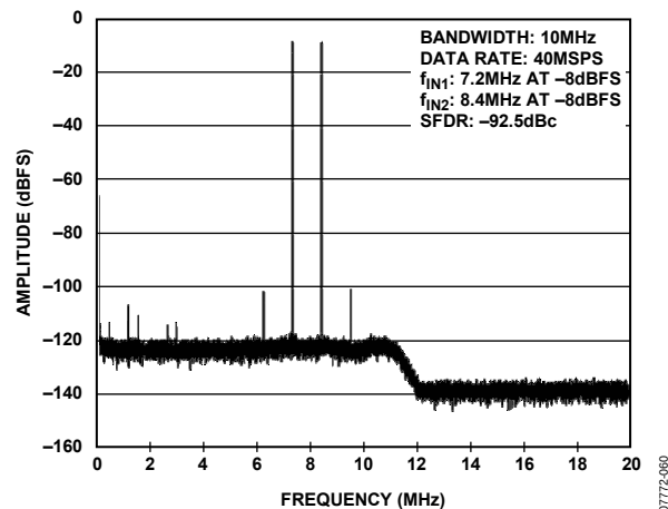
Figure 21. AD9262BCPZ-10 Two-Tone FFT with f_{IN1} = 7.2 MHz, f_{IN2} = 8.4 MHz
