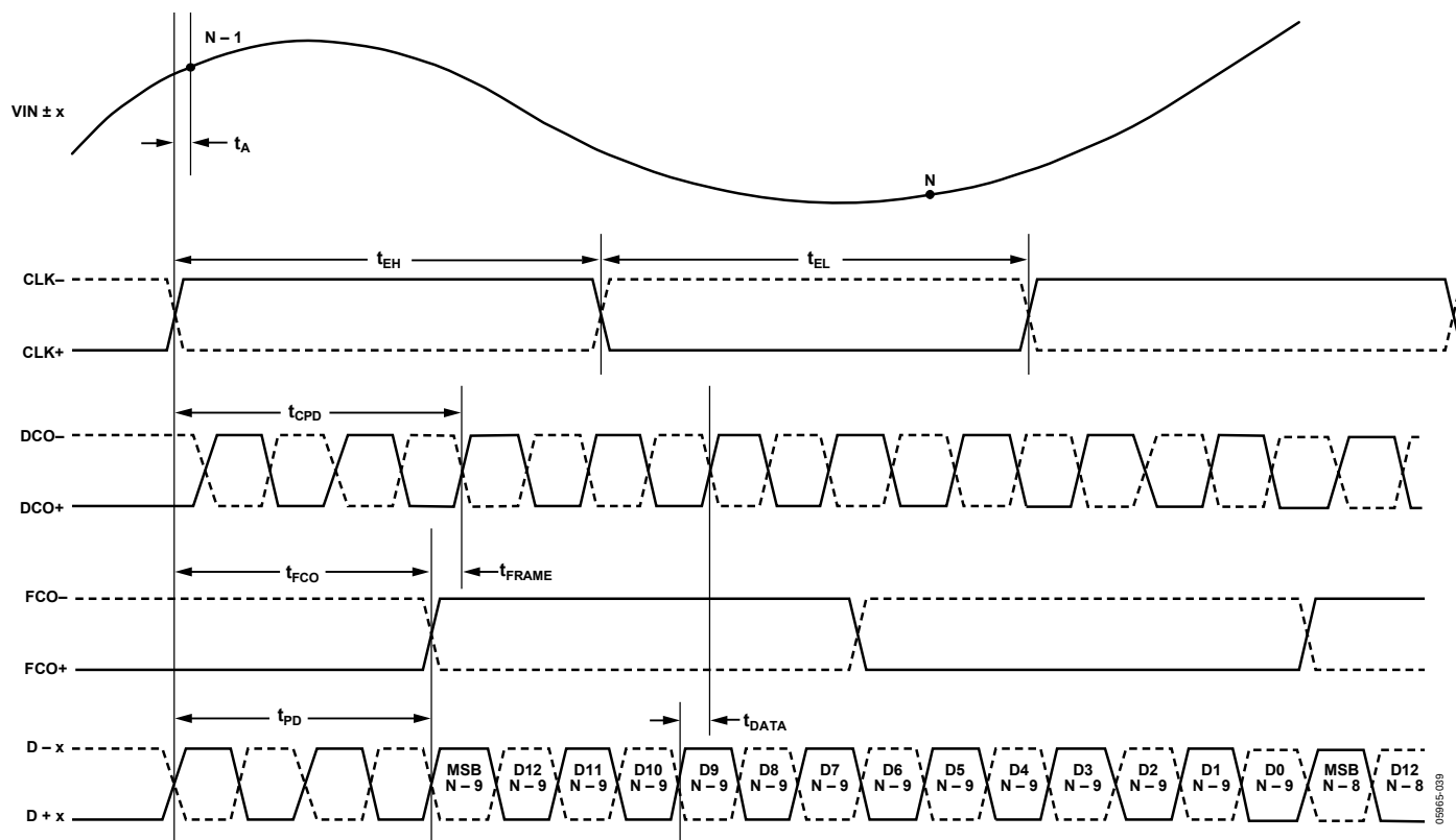
Figure 2. 14-Bit Data Serial Stream, MSB First (Default)
