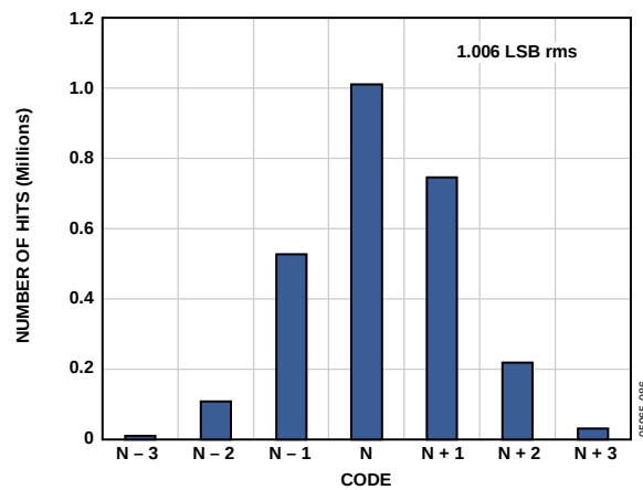
Figure 32. Input-Referred Noise Histogram, f_{\text{SAMPLE}} = 50 \text{ MSPS}
