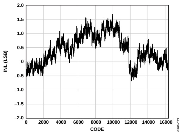
Figure 29. INL, f_{\text{IN}} = 2.4 \text{ MHz} , f_{\text{SAMPLE}} = 50 \text{ MSPS}
