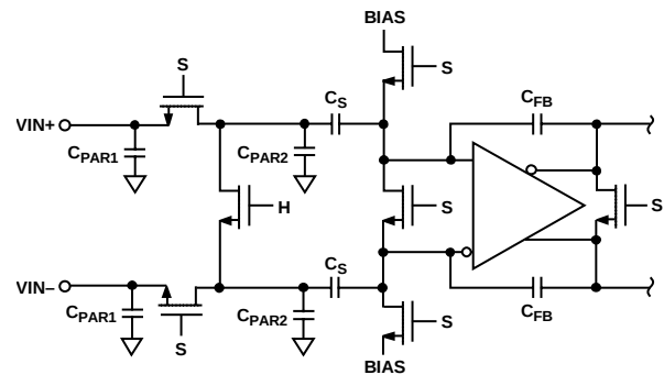
Figure 64. Switched-Capacitor Input
