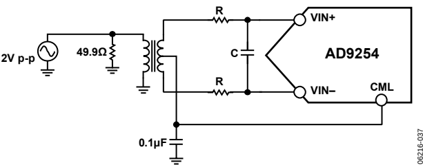
Figure 33. Differential Transformer-Coupled Configuration
