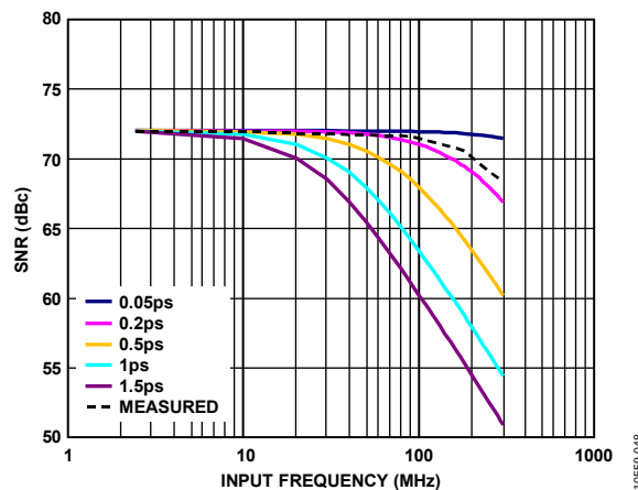
Figure 52. AD9250-250 SNR vs. Input Frequency and Jitter
