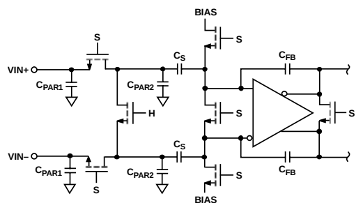
Figure 38. Switched-Capacitor Input
