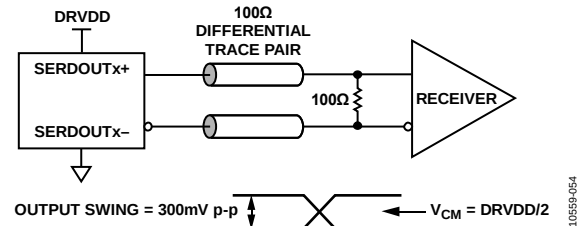
Figure 54. DC-Coupled Digital Output Termination Example
