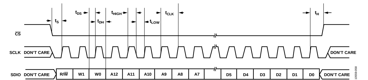
Figure 58. Serial Port Interface Timing Diagram
