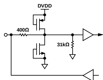
Figure 31. Equivalent SDIO Circuit
