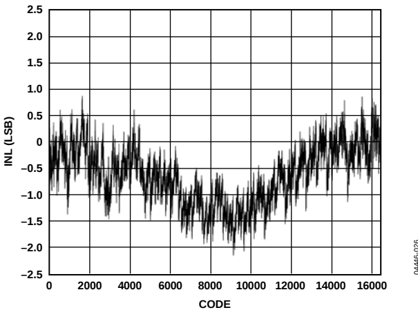
Figure 27. AD9248-65 Typical INL
