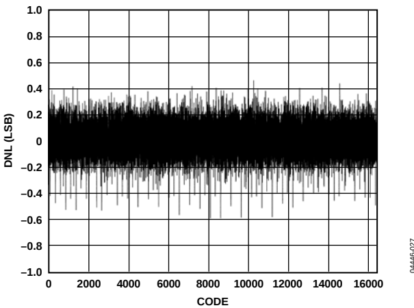
Figure 28. AD9248-65 Typical DNL
