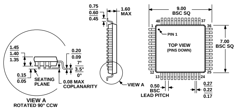
COMPLIANT TO JEDEC STANDARDS MS-026-BBC Figure 74. 48-Lead Low Profile Quad Flat Package [LQFP] (ST-48) Dimensions shown in millimeters
