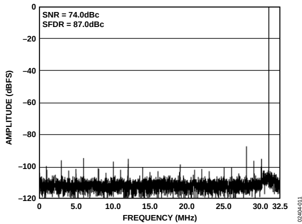
Figure 11. Single-Tone FFT, f_{\text{IN}} = 31 MHz
