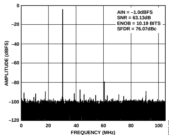
Figure 7. Single-Tone 32k FFT with f_{IN} = 240.3 MHz, f_{SAMPLE} = 210 MSPS
