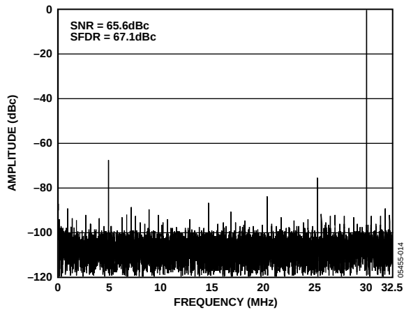
Figure 14. AD9237-65 100 MHz FFT
