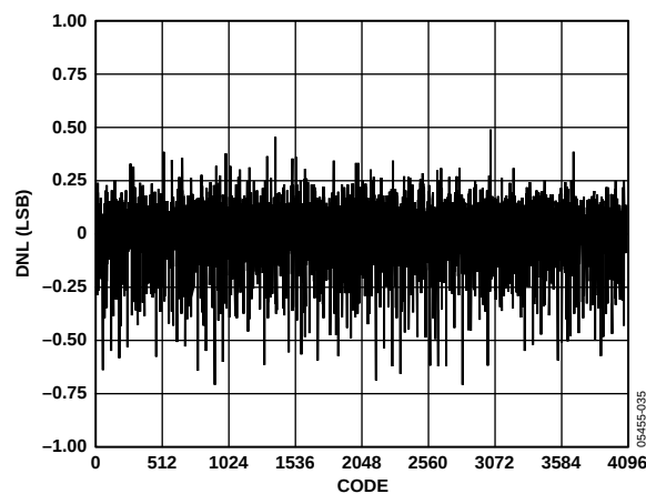
Figure 31. Typical DNL
