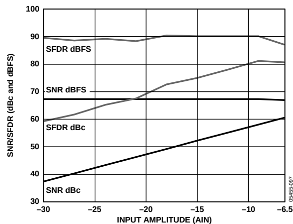
Figure 29. AD9237-40 Two-Tone SNR/SFDR vs. Analog Input with f_{IN1} = 69 \text{ MHz} , f_{IN2} = 70 \text{ MHz}
