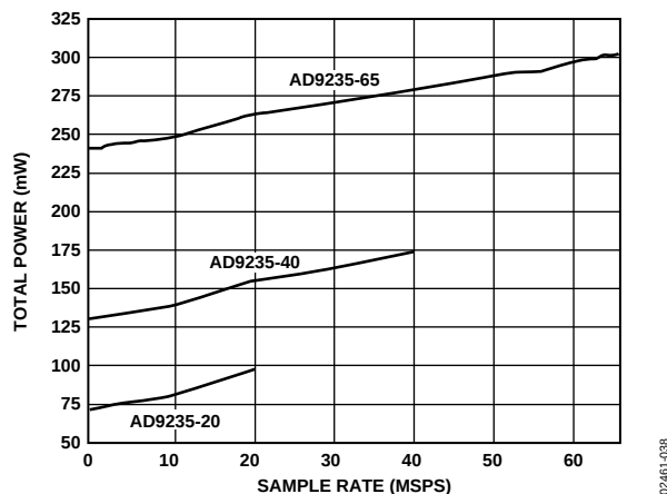
Figure 38. Total Power vs. Sample Rate with f_{\text{IN}} = 10 \text{ MHz}
