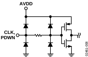
Figure 8. Equivalent Digital Input Circuit
