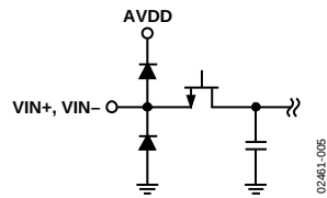
Figure 5. Equivalent Analog Input Circuit
