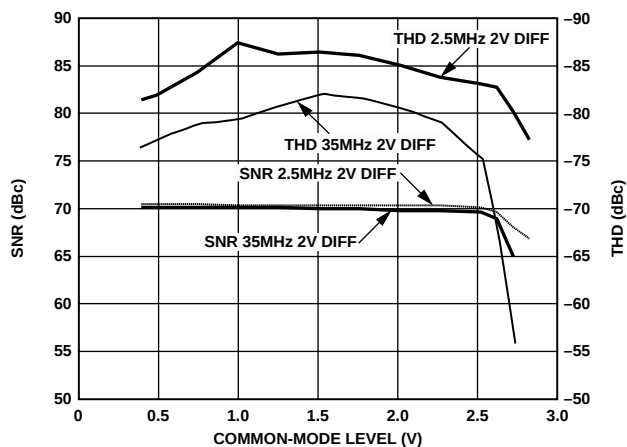
Figure 34. AD9235-65: SNR, THD vs. Common-Mode Level
