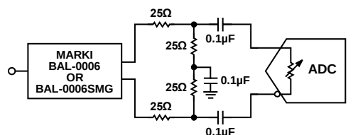
Figure 64. Differential Transformer-Coupled Configuration for Frequencies > 500 MHz
