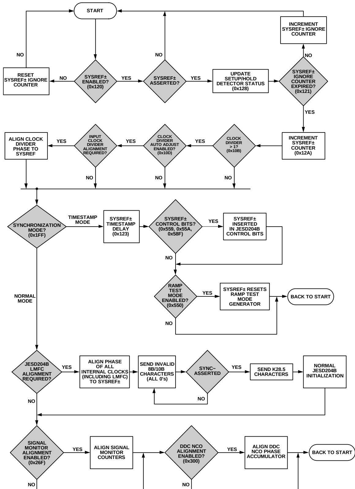
Figure 103. Multichip Synchronization
