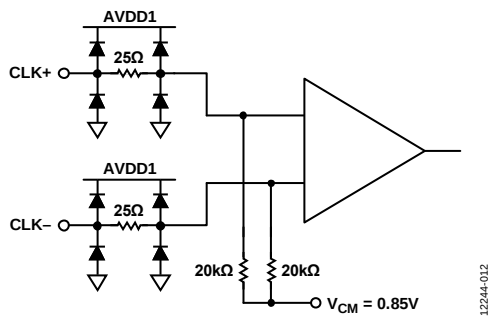
Figure 53. Clock Inputs
