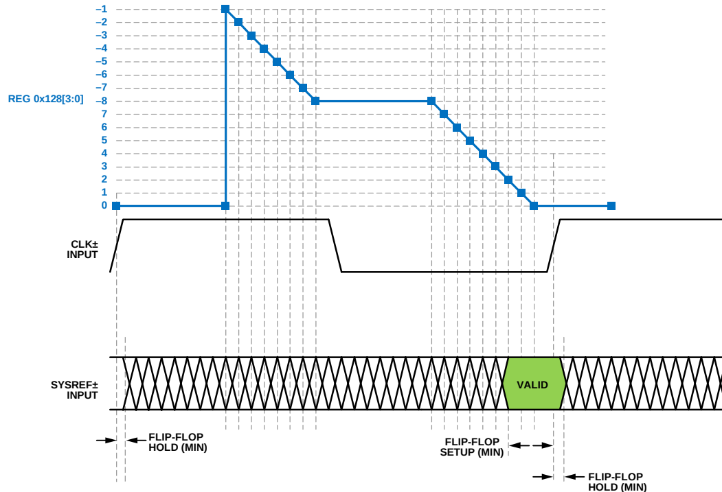
Figure 104. SYSREF± Setup Detector
