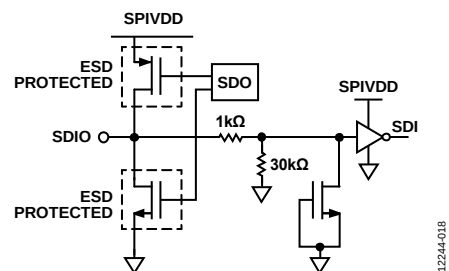
Figure 59. SDIO Input
