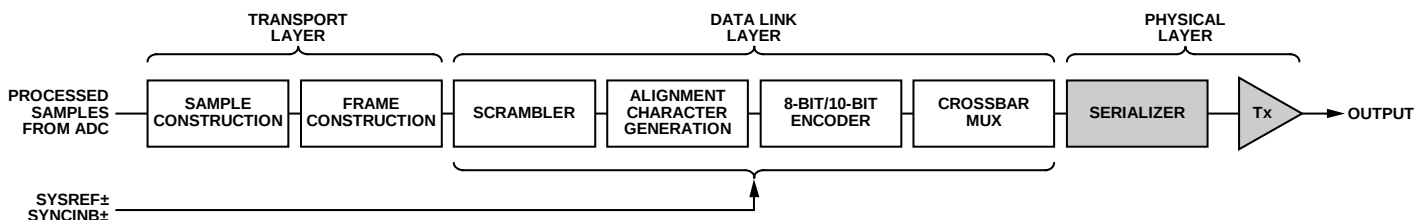
Figure 92. Data Flow
