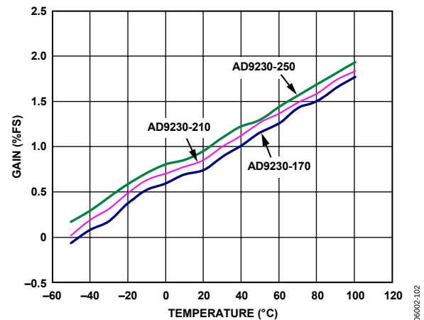
Figure 50. Gain vs. Temperature
