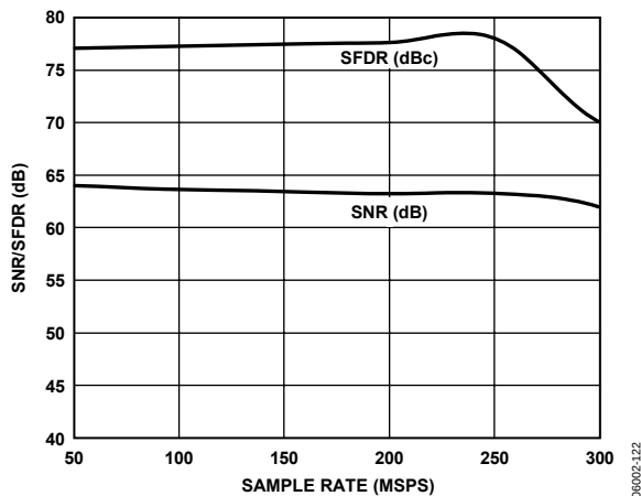
Figure 47. SNR/SFDR vs. Sample Rate; 250 MSPS, 170.3 MHz @ -1 dBFS
