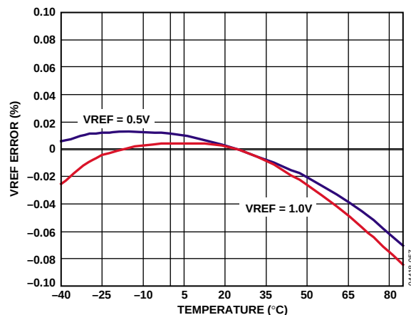
Figure 45. Typical VREF Drift
