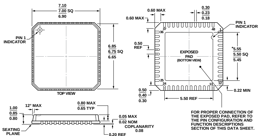
*COMPLIANT TO JEDEC STANDARDS MO-220-VKGD-2 WITH EXCEPTION TO EXPOSED PAD DIMENSION. Figure 58. 48-Lead Lead Frame Chip Scale Package [LFCSP_VQ] 7 mm × 7 mm Body, Very Thin Quad (CP-48-8) Dimensions shown in millimeters
