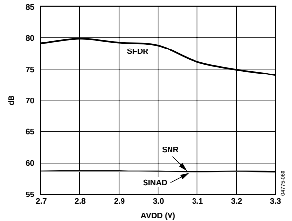
Figure 33. SNR, SINAD, SFDR vs. AVDD, A_{IN} = 70 MHz at -0.5 dBFS, 65 MSPS (-65 Grade)
