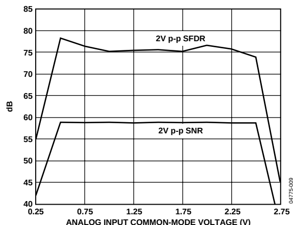
Figure 42. Input Common-Mode Voltage Sensitivity
