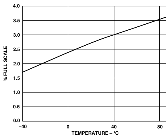
TPC 14. ADC Gain vs. Temperature (with External 1.25 \text{ V} Reference)
