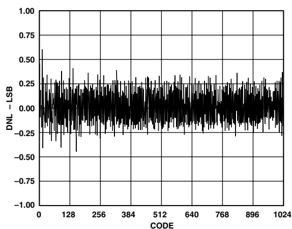
TPC 18. DNL @ 80 \text{ MSPS}
