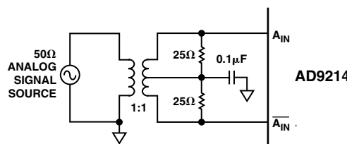
Figure 8. Single-Ended-to-Differential Conversion Using a Transformer
