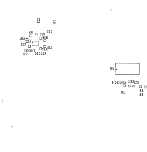
Figure 13. PCB Bottom Side Silkscreen
