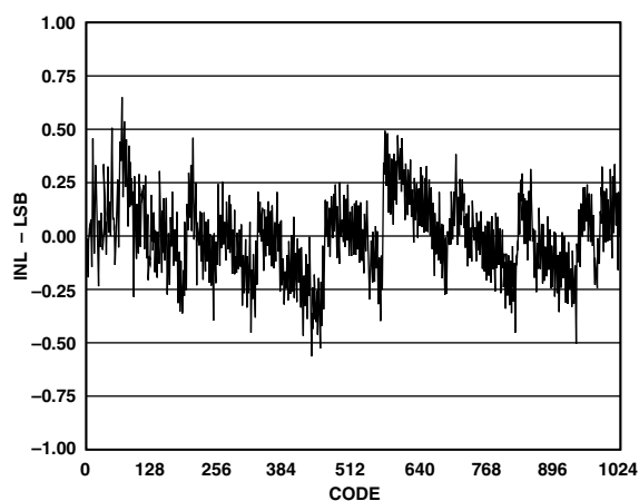
TPC 17. INL @ 80 \text{ MSPS}
