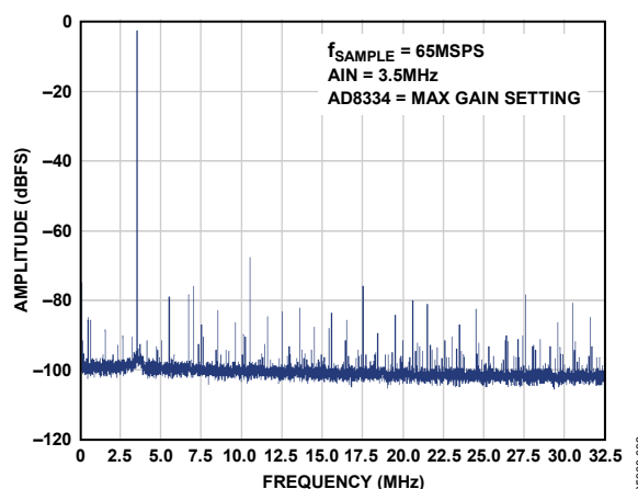
Figure 73. AD9212 FFT Example Results Using 16 MHz, Two-Pole Low-Pass Filter Applied to the AD8334 Outputs (Analog Input Signal = -1.03 dBFS, SNR = 56.75 dBc, SFDR = 64.4 dBc)
