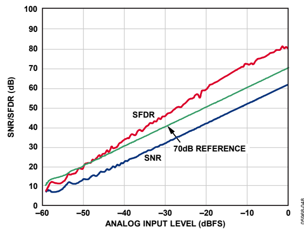
Figure 26. SNR/SFDR vs. Analog Input Level, f_{\text{IN}} = 35 MHz, AD9212-40
