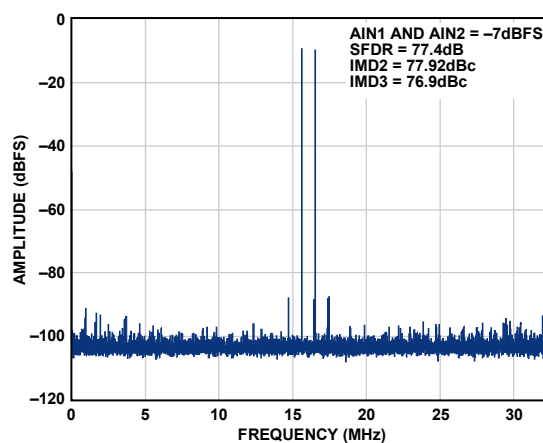
Figure 31. Two-Tone 32k FFT with f_{IN1} = 15 MHz and f_{IN2} = 16 MHz, AD9212-65
