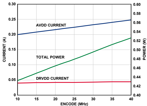
Figure 57. Supply Current vs. f_{\text{SAMPLE}} for f_{\text{IN}} = 10.3 MHz, AD9212-40
