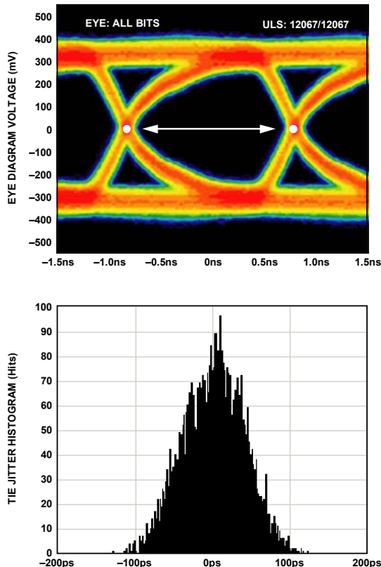
Figure 61. Data Eye for LVDS Outputs in ANSI-644 Mode with Trace Lengths Greater Than 24 Inches on Standard FR-4
