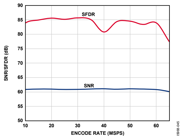
Figure 23. SNR/SFDR vs. f_{\text{SAMPLE}} , f_{\text{IN}} = 10.3 MHz, AD9212-65
