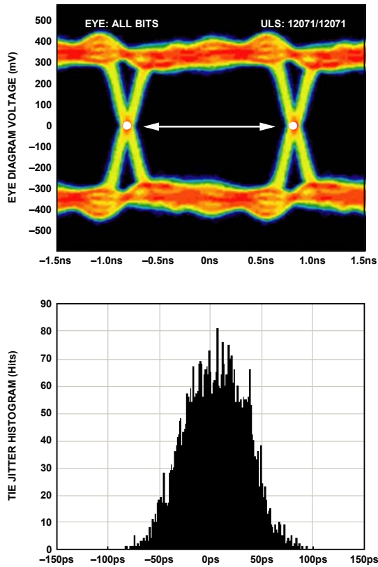
Figure 60. Data Eye for LVDS Outputs in ANSI-644 Mode with Trace Lengths Less Than 24 Inches on Standard FR-4
