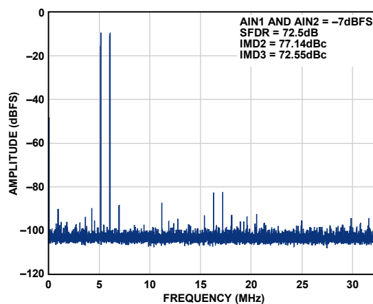
Figure 32. Two-Tone 32k FFT with f_{IN1} = 70 MHz and f_{IN2} = 71 MHz, AD9212-65
