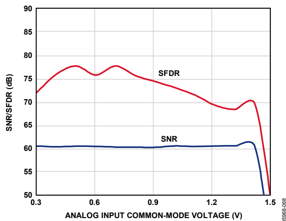
Figure 46. SNR/SFDR vs. Common-Mode Voltage, f_{IN} = 35 MHz, AD9212-65
