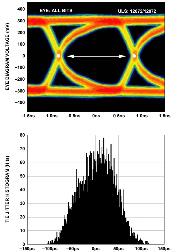
Figure 62. Data Eye for LVDS Outputs in ANSI-644 Mode with 100 \Omega Termination On and Trace Lengths Greater Than 24 Inches on Standard FR-4
