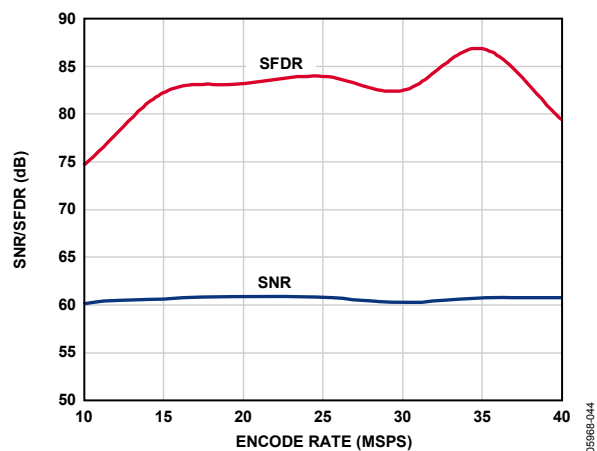
Figure 22. SNR/SFDR vs. f_{\text{SAMPLE}} , f_{\text{IN}} = 19.7 MHz, AD9212-40
