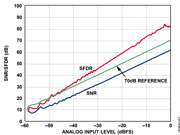
Figure 25. SNR/SFDR vs. Analog Input Level, f_{\text{IN}} = 10.3 MHz, AD9212-40
