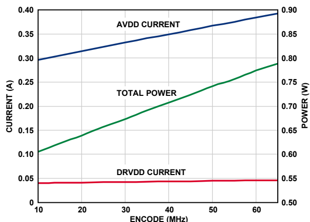
Figure 58. Supply Current vs. f_{\text{SAMPLE}} for f_{\text{IN}} = 10.3 MHz, AD9212-65
