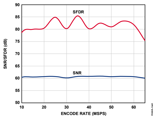
Figure 24. SNR/SFDR vs. f_{\text{SAMPLE}} , f_{\text{IN}} = 35 MHz, AD9212-65
