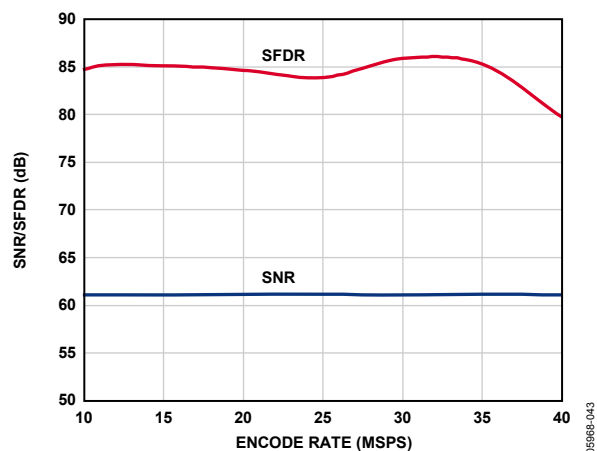
Figure 21. SNR/SFDR vs. f_{\text{SAMPLE}} , f_{\text{IN}} = 10.3 MHz, AD9212-40
