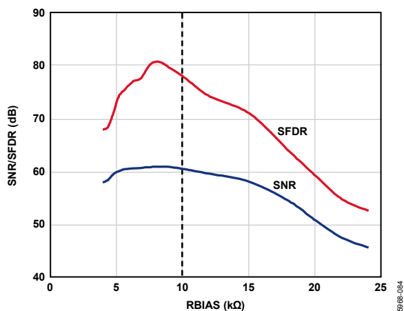
Figure 65. SNR/SFDR vs. RBIAS, AD9212-65
