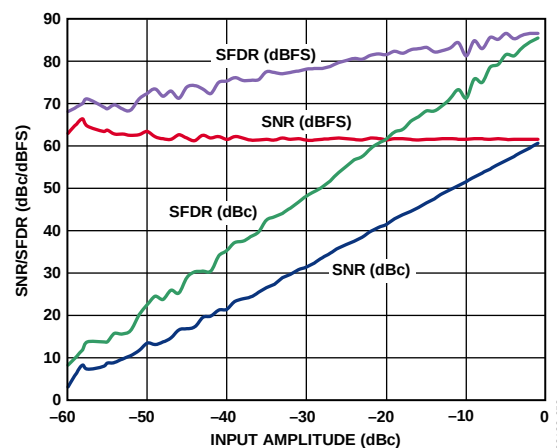
Figure 28. AD9204-20 SNR/SFDR vs. Input Amplitude ( A_{IN} ) with f_{IN} = 9.7 MHz
