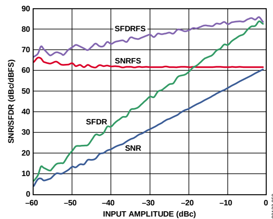
Figure 25. AD9204-40 SNR/SFDR vs. Input Amplitude (AIN) with f_{IN} = 9.7 MHz
