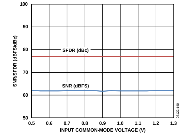
Figure 40. SNR/SFDR vs. Input Common-Mode Voltage, f_{IN} = 10.3\text{ MHz} , f_s = 20\text{ MSPS}
