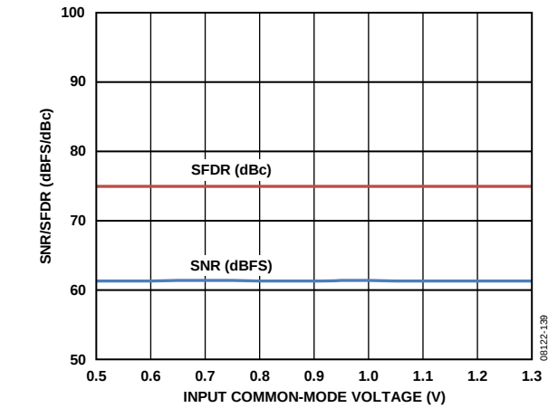
Figure 39. SNR/SFDR vs. Input Common-Mode Voltage, f_{IN} = 32.1\text{ MHz} , f_s = 80\text{ MSPS}
