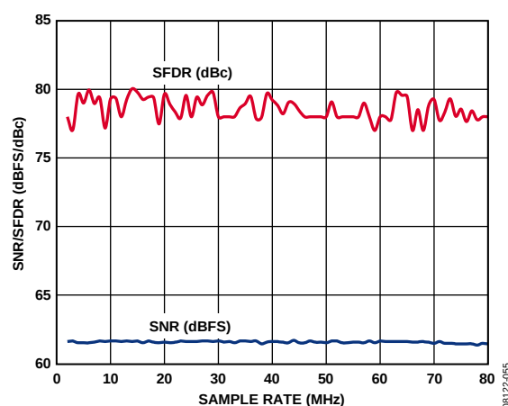
Figure 13. AD9204-80 SNR/SFDR vs. Sample Rate with f_{IN} = 9.7 MHz
