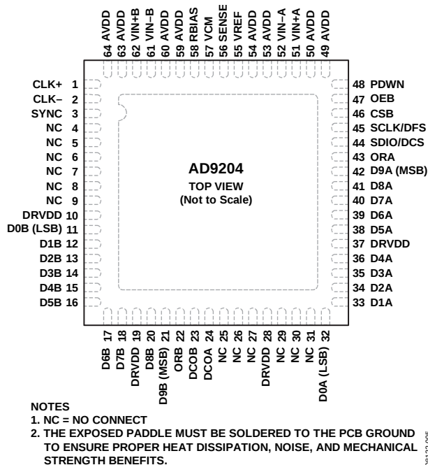
Figure 5. Pin Configuration
