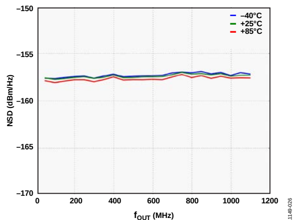
Figure 22. W-CDMA NSD vs. f_{OUT} over Temperature
