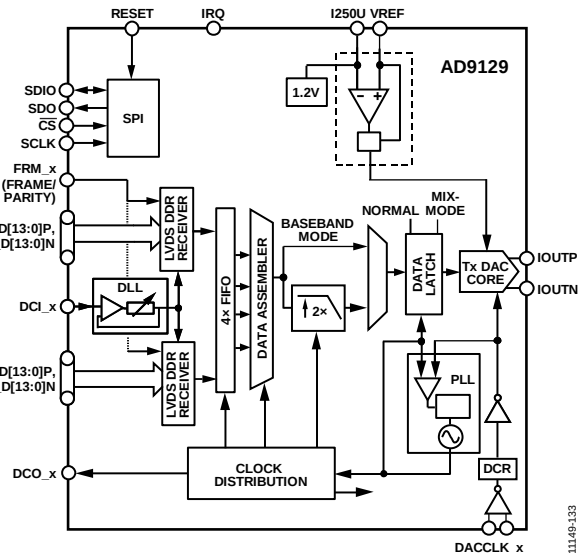
Figure 128. Functional Block Diagram of the AD9119/AD9129
