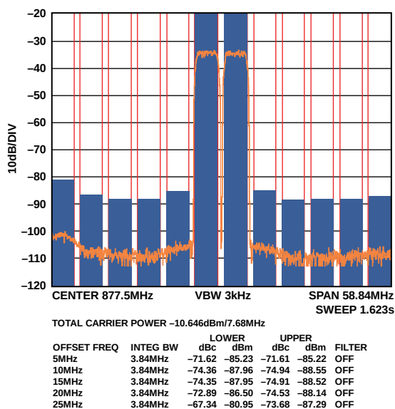
Figure 23. Two-Carrier W-CDMA at 877.5 MHz
