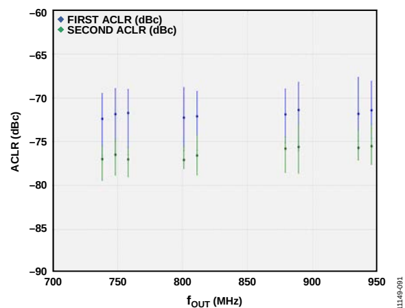
Figure 82. Two-Carrier W-CDMA ACLR vs. f_{OUT} (First ACLR, Second ACLR)
