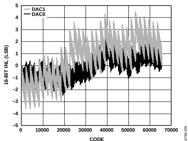
Figure 40. INL, I_{OUTFS} = 26 mA, 16-Bit Resolution
