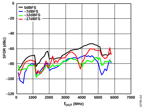
Figure 21. Third Harmonic (SFDR) vs. f_{OUT} over Digital Scale (Mode 10), 12 GHz DAC Sample Rate, Channel Interpolation 1 \times , Main Interpolation 4 \times
