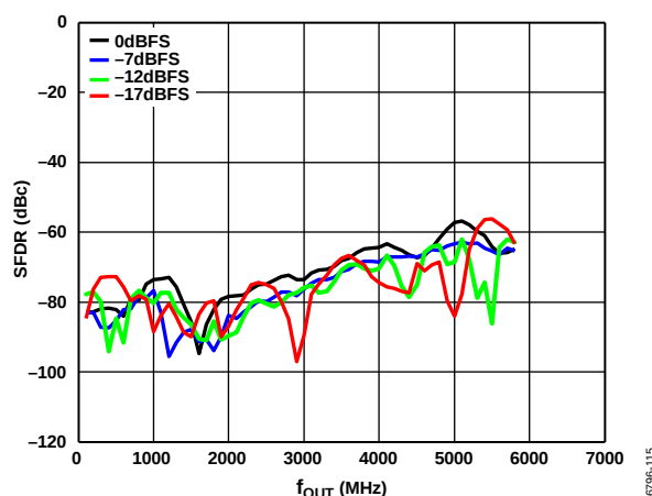
Figure 18. Second Harmonic (SFDR) vs. f_{OUT} over Digital Scale (Mode 9), 12 GHz DAC Sample Rate, Channel Interpolation 1 \times , Main Interpolation 8 \times
