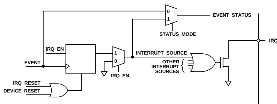
Figure 87. Simplified Schematic of \overline{IRQx} Circuitry
