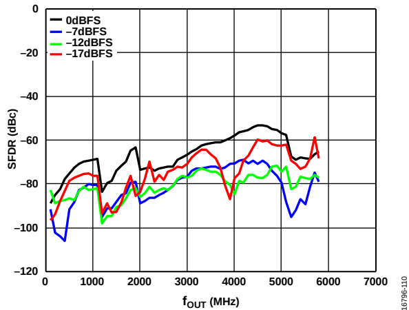
Figure 10. Third Harmonic (SFDR) vs. f_{OUT} over Digital Scale (Mode 2), 12 GHz DAC Sample Rate, Channel Interpolation 4x, Main Interpolation 8x
