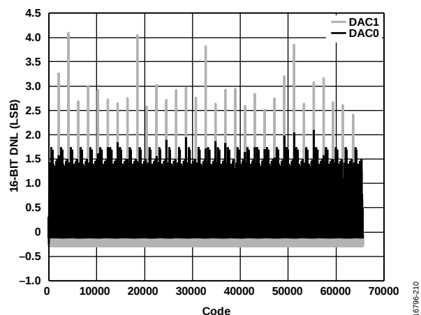
Figure 41. DNL, I_{OUTFS} = 20 mA, 16-Bit Resolution
