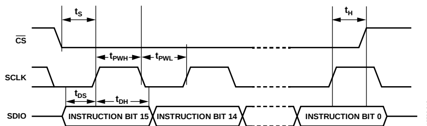
Figure 51. Timing Diagram for Serial Port Register Write
