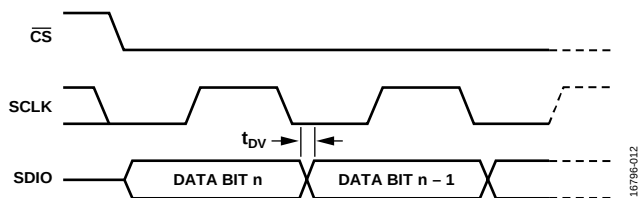
Figure 50. Timing Diagram for Serial Port Register Read
