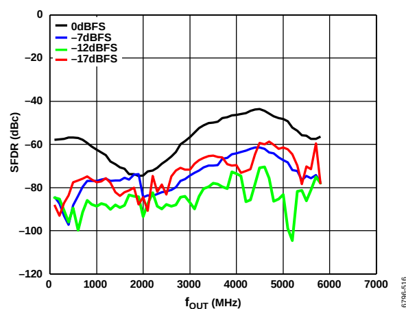
Figure 19. Third Harmonic (SFDR) vs. f_{OUT} over Digital Scale (Mode 9), 12 GHz DAC Sample Rate, Channel Interpolation 1 \times , Main Interpolation 8 \times
