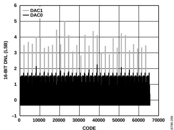
Figure 39. DNL, I_{OUTFS} = 26 mA, 16-Bit Resolution
