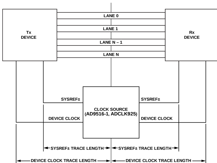
Figure 97. SYSREF \pm Signal and Device Clock Trace Length
