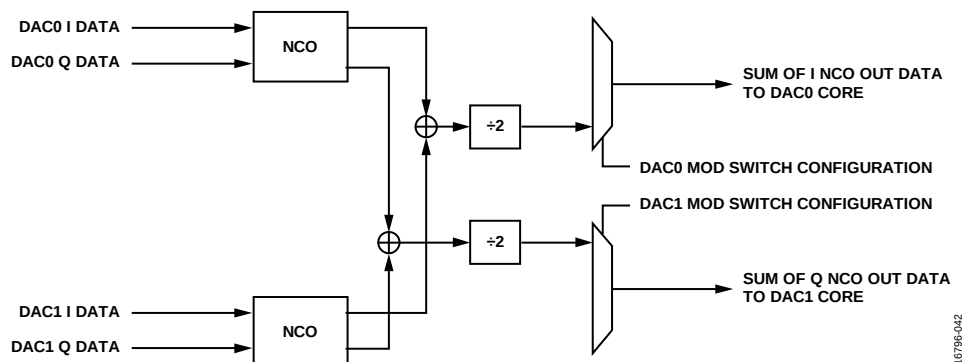
Figure 82. Configuration 1, CMPLX_MOD_DIV2_DISABLE = 0—DAC0 = I0 + I1, DAC1 = Q0 + Q1
