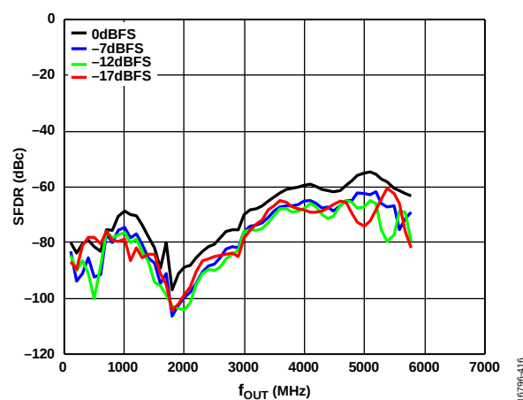
Figure 20. Second Harmonic (SFDR) vs. f_{OUT} over Digital Scale (Mode 10), 12 GHz DAC Sample Rate, Channel Interpolation 1 \times , Main Interpolation 4 \times
