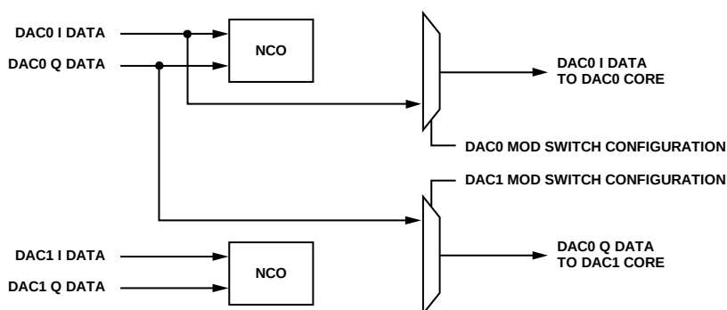
Figure 83. Configuration 2—DAC0 = I0, DAC1 = Q0
