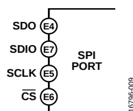
Figure 47. Serial Port Interface Pins (144-Ball BGA_ED)
