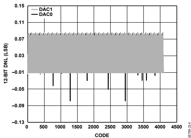
Figure 45. DNL, I_{OUTFS} = 20 mA, 12-Bit Resolution
