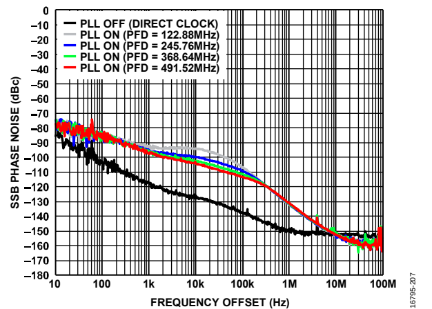
Figure 37. Single-Sideband (SSB) Phase Noise vs. Offset over f_{OUT} , over PFD Frequency, f_{DAC} = 12 GHz, f_{OUT} = 1.8 GHz, PLL On, PLL Reference Clock = 500 MHz
