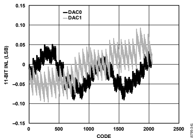
Figure 48. INL, I_{OUTFS} = 20 mA, 11-Bit Resolution
