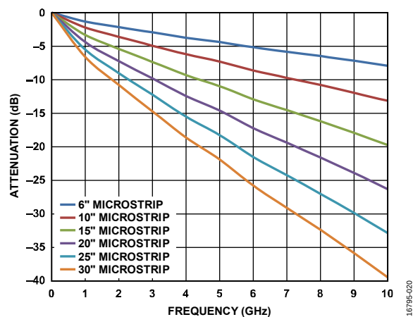
Figure 60. Insertion Loss of 50 \Omega Microstrips on FR4
