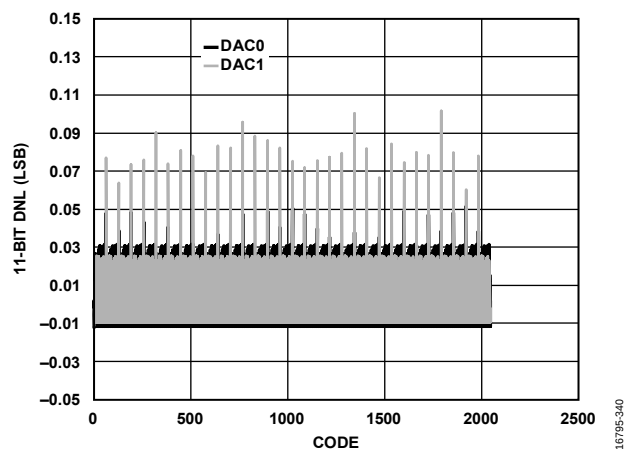
Figure 47. DNL, I_{OUTFS} = 20 mA, 11-Bit Resolution
