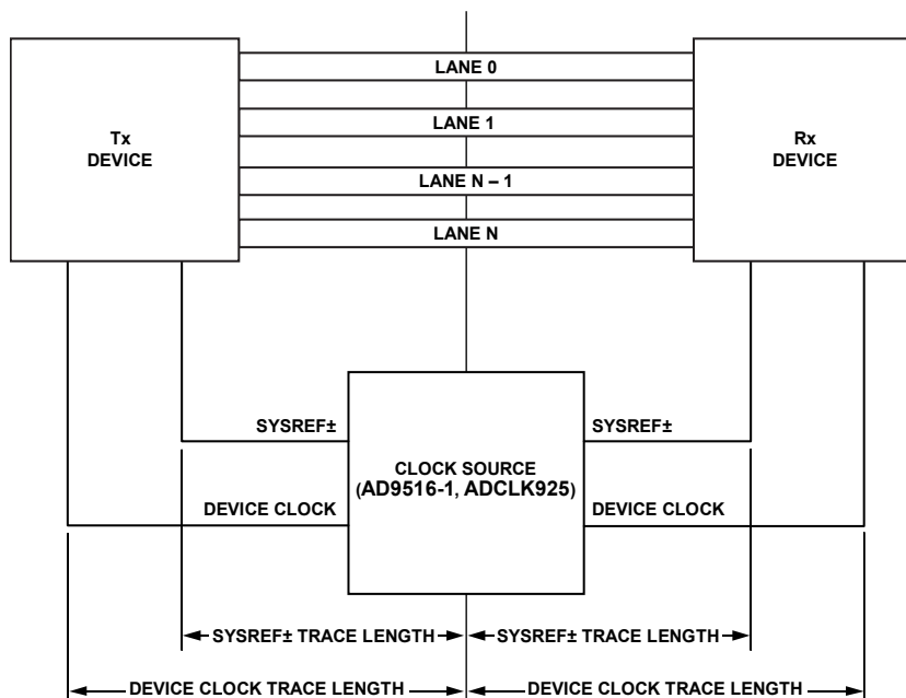
Figure 99. SYSREF \pm Signal and Device Clock Trace Length
