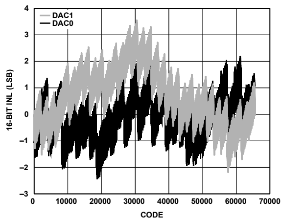
Figure 44. INL, I_{OUTFS} = 15.6 mA, 16-Bit Resolution
