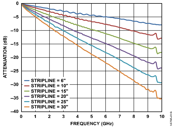
Figure 59. Insertion Loss of 50 \Omega Striplines on FR4
