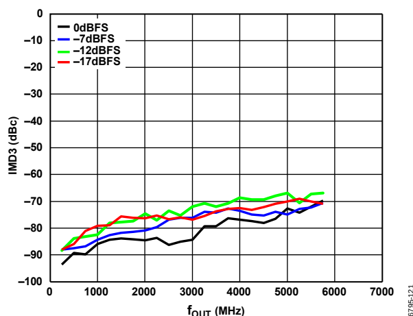
Figure 24. IMD3 vs. f_{OUT} over Digital Scale (Mode 2), 12 GHz DAC Sample Rate, Channel Interpolation 4 \times , Main Interpolation 8 \times , 1 MHz Tone Spacing
