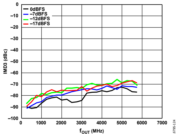
Figure 27. IMD3 vs. f_{OUT} over Digital Scale (Mode 9), 12 GHz DAC Sample Rate, Channel Interpolation 1 \times , Main Interpolation 12 \times , 1 MHz Tone Spacing
