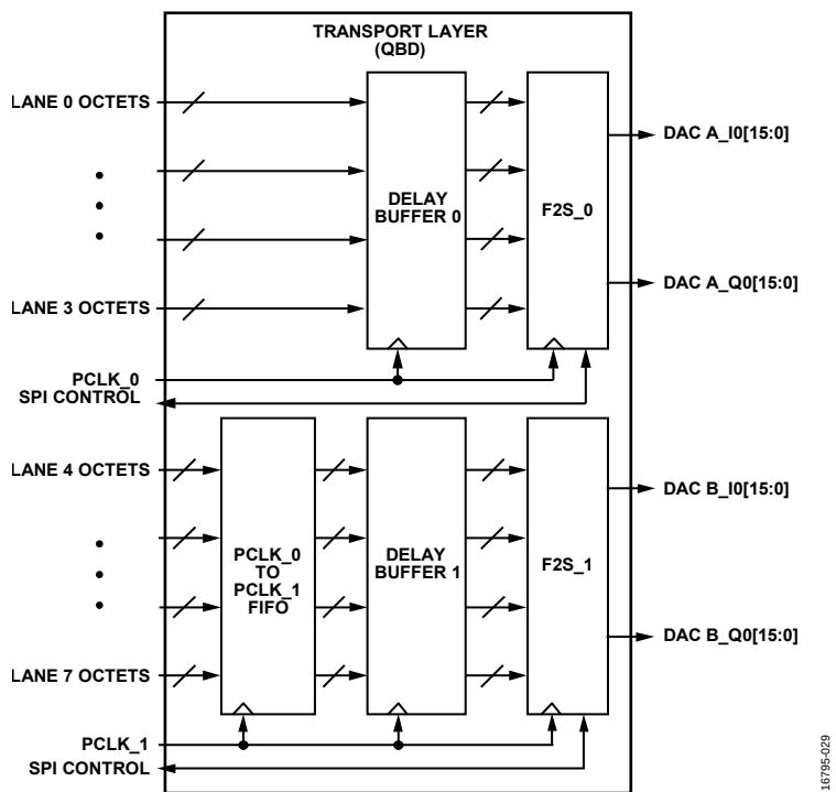
Figure 71. Transport Layer Block Diagram
