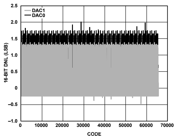
Figure 43. DNL, I_{OUTFS} = 15.6 mA, 16-Bit Resolution
