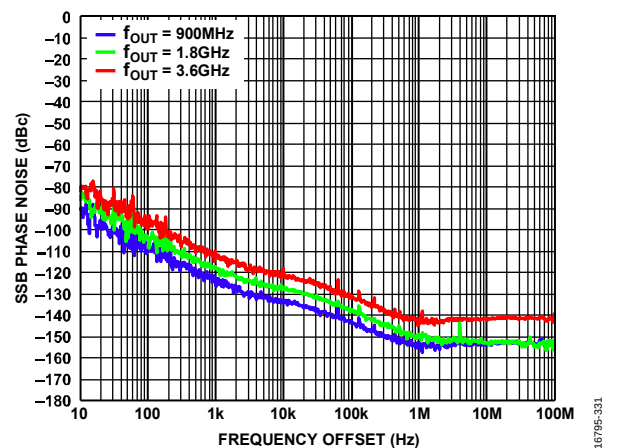
Figure 38. SSB Phase Noise vs. Frequency Offset over f_{OUT} , f_{DAC} = 12 GHz, Direct Clock (PLL Off)
