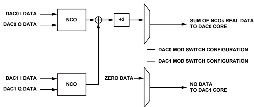
Figure 86. Configuration 3, CMLX\_MOD\_DIV2\_DISABLE = 0 — DAC0 = I0 + I1 , DAC1 = 0
