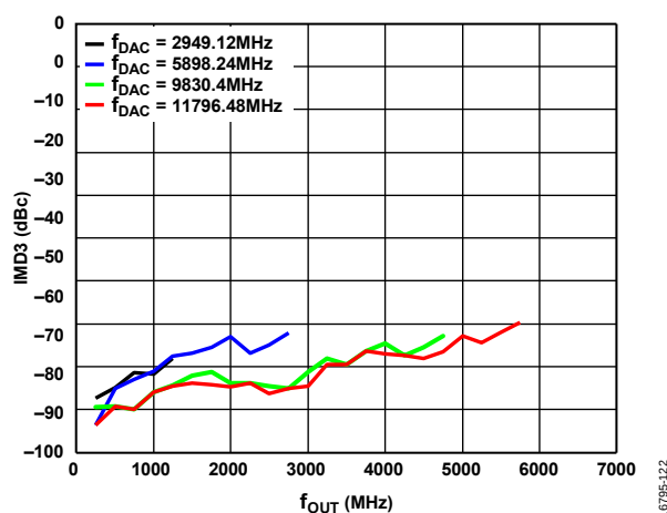
Figure 25. IMD3 vs. f_{OUT} over f_{DAC} (Mode 2), Channel Interpolation 4 \times , Main Interpolation 8 \times , 1 MHz Tone Spacing
