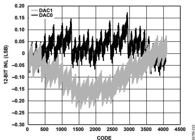
Figure 46. INL, I_{OUTFS} = 20 mA, 12-Bit Resolution
