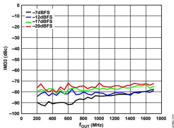
Figure 26. IMD3 vs. f_{OUT} over Digital Scale (Mode 17), 3.4 GHz DAC Sample Rate, Channel Interpolation 1 \times , Main Interpolation 1 \times , 1 MHz Tone Spacing, 11-Bit Resolution
