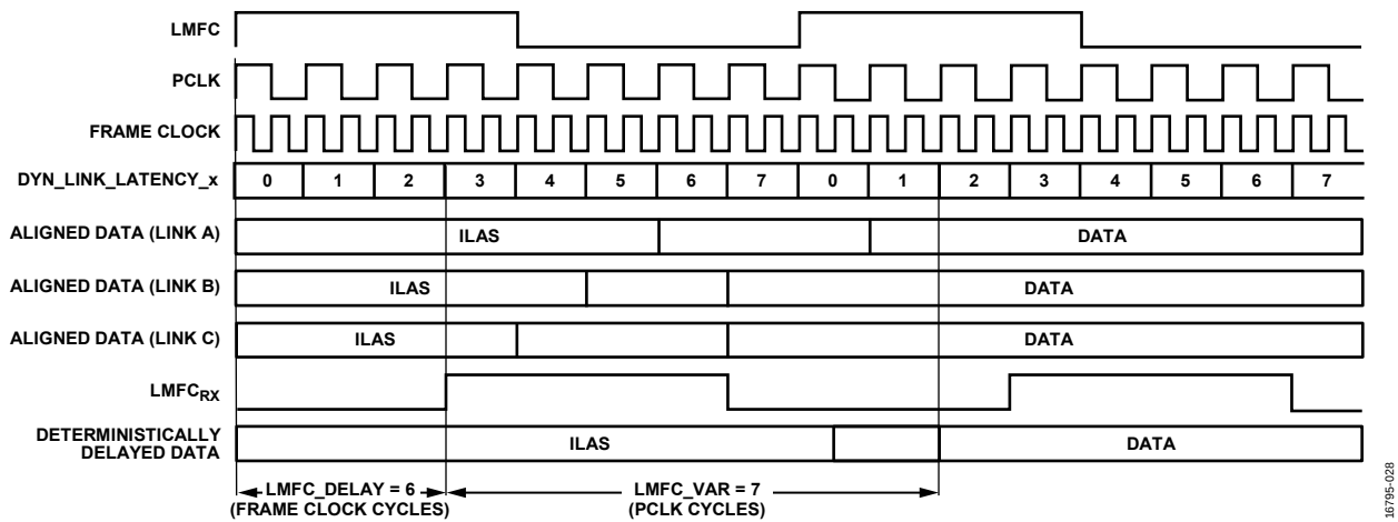
Figure 70. Multilink Synchronization Settings, Derived Method Example
