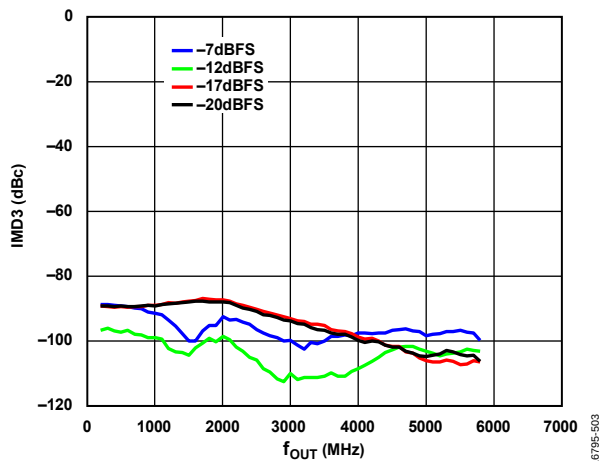
Figure 28. Worst IMD3 vs. f_{OUT} over Digital Scale (Mode 23), 12 GHz DAC Sample Rate, Channel Interpolation 1 \times , Main Interpolation 6 \times , 1 MHz Tone Spacing
