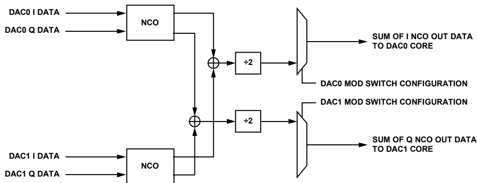
Figure 84. Configuration 1, CMLX\_MOD\_DIV2\_DISABLE = 0 — DAC0 = I0 + I1 , DAC1 = Q0 + Q1
