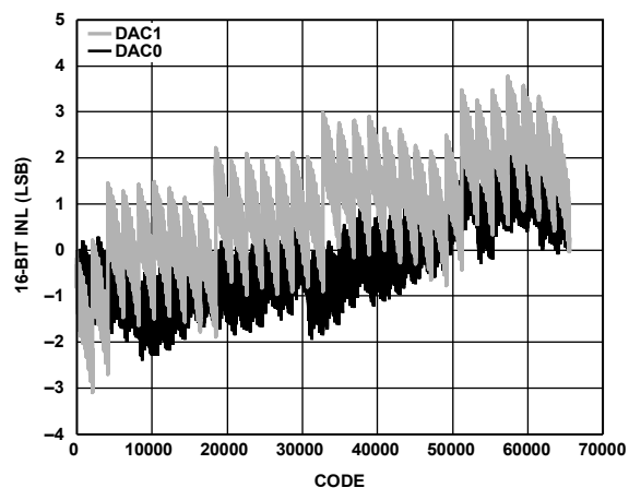
Figure 42. INL, I_{OUTFS} = 20 mA, 16-Bit Resolution
