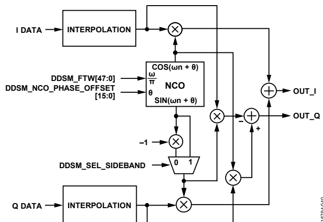
Figure 79. NCO Modulator Block Diagram, Main Datapath Modulus NCO Mode (DDS)
