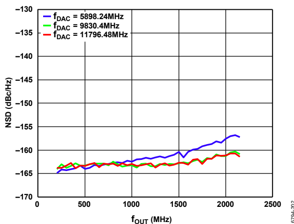
Figure 32. NSD vs. f_{OUT} over f_{DAC} , 16-Bit Resolution, Shuffle On, Single Tone Measured at 70 MHz
