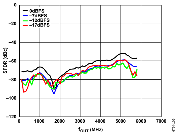
Figure 9. Second Harmonic (SFDR) vs. f_{OUT} over Digital Scale (Mode 2), 12 GHz DAC Sample Rate, Channel Interpolation 4 \times , Main Interpolation 8 \times
