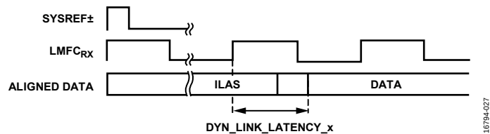
Figure 67. DYN_LINK_LATENCY_x Illustration
