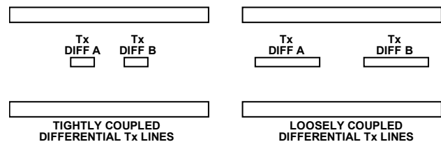
Figure 96. Tightly Coupled vs. Loosely Coupled Differential Traces
