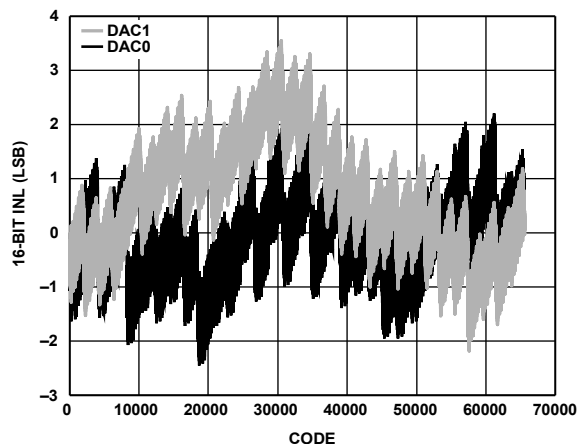
Figure 38. INL, I_{OUTFS} = 15.6 mA, 16-Bit Resolution
