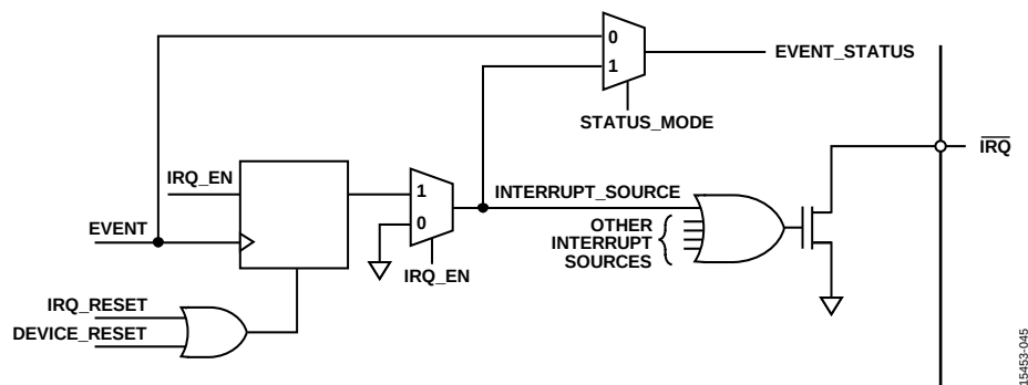
Figure 79. Simplified Schematic of \overline{\text{IRQx}} Circuitry
