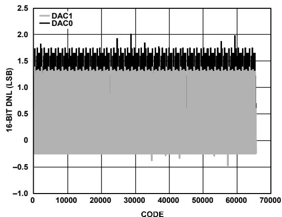
Figure 37. DNL, I_{OUTFS} = 15.6 mA, 16-Bit Resolution
