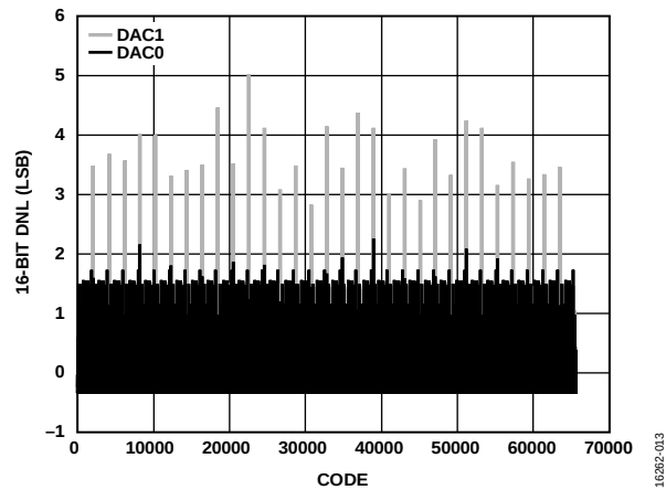
Figure 14. DNL, I_{OUTFS} = 26 mA, 16-Bit Resolution
