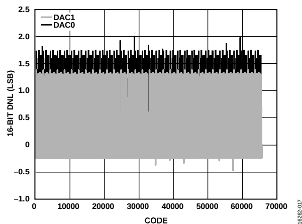
Figure 18. DNL, I_{OUTFS} = 15.6 mA, 16-Bit Resolution
