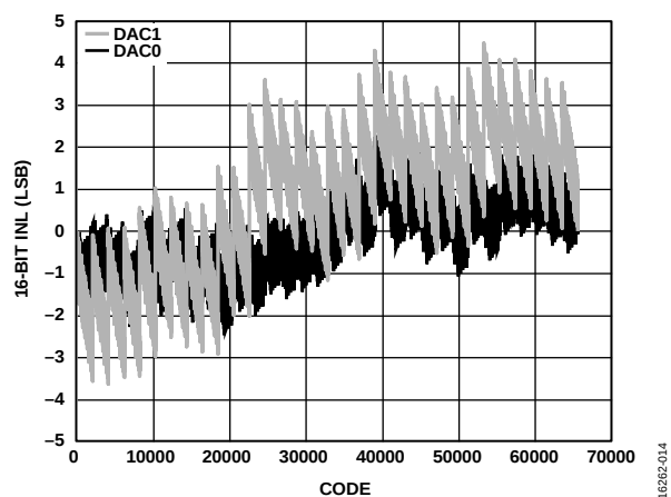
Figure 15. INL, I_{OUTFS} = 26 mA, 16-Bit Resolution
