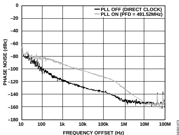
Figure 65. Phase Noise vs. Frequency Offset; Direct Clock and PLL Phase Noise, 12 GHz DAC Sample Rate, 1.65 GHz Output Frequency
