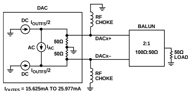
Figure 67. Equivalent DAC Output Circuit and Recommended DAC Output Network
