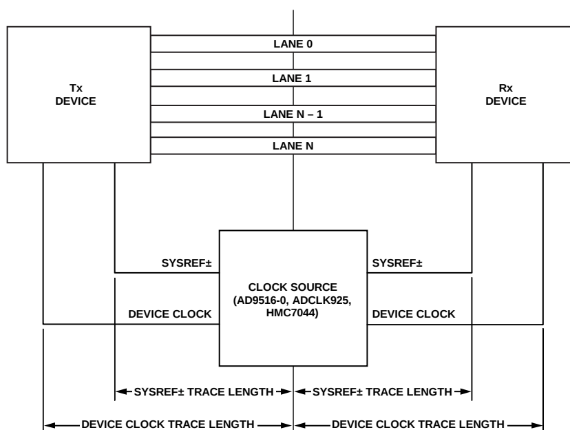
Figure 63. SYSREF \pm Signal and Device Clock Trace Length
