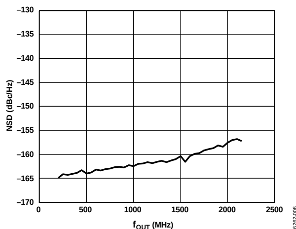
Figure 8. Single-Tone NSD Measured at 70 MHz vs. f_{OUT} , f_{DAC} = 5.89824\text{GHz} , 16-Bit Resolution, Shuffle On
