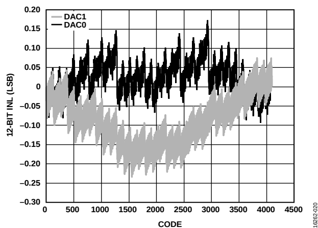
Figure 21. INL, I_{OUTFS} = 20 \text{ mA} , 12-Bit Resolution
