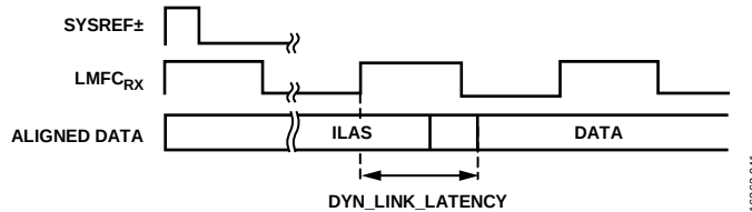
Figure 42. DYN_LINK_LATENCY_x Illustration
