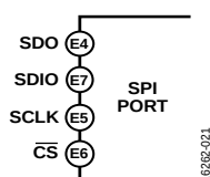
Figure 22. Serial Port Interface Pins (144-Ball BGA_ED)
