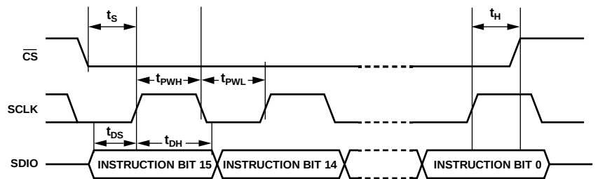
Figure 26. Timing Diagram for Serial Port Register Write
