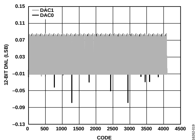
Figure 20. DNL, I_{OUTFS} = 20 \text{ mA} , 12-Bit Resolution
