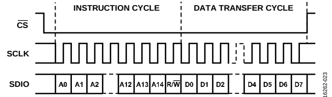
Figure 24. Serial Register Interface Timing, LSB First, Register 0x000, Bit 6 and Bit 1 = 1
