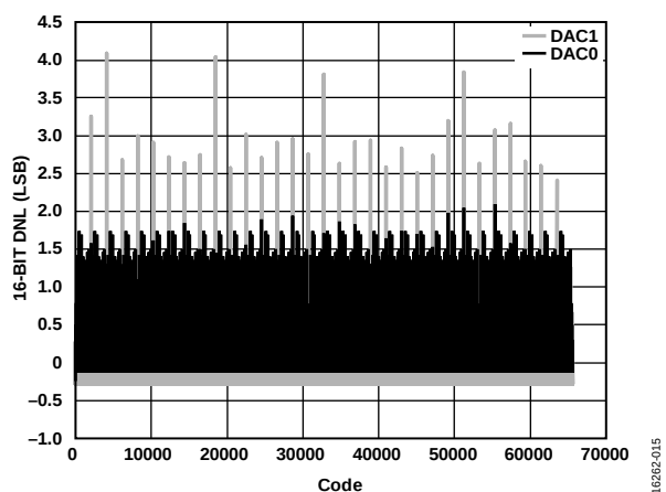
Figure 16. DNL, I_{OUTFS} = 20 mA, 16-Bit Resolution
