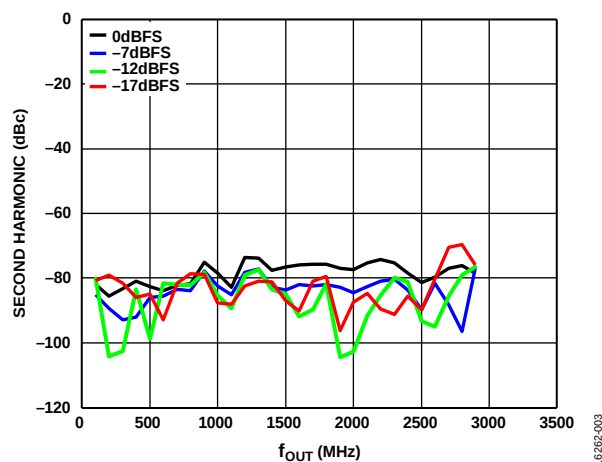
Figure 3. Second Harmonic (dBc) vs. f_{OUT} over Digital Scale (Mode 0), 6 GHz DAC Sample Rate, Channel Interpolation 2 \times , Main Interpolation 8 \times
