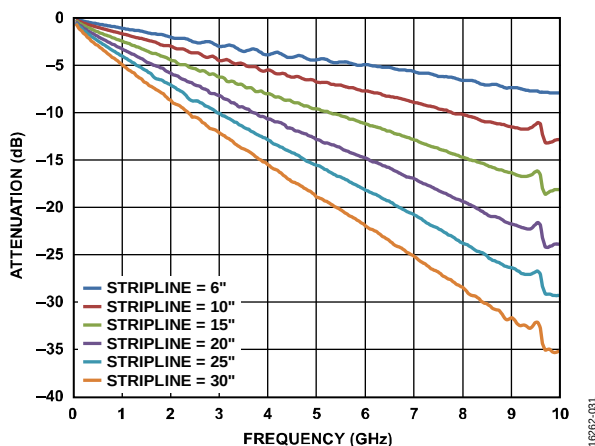
Figure 32. Insertion Loss of 50 \Omega Striplines on FR4
