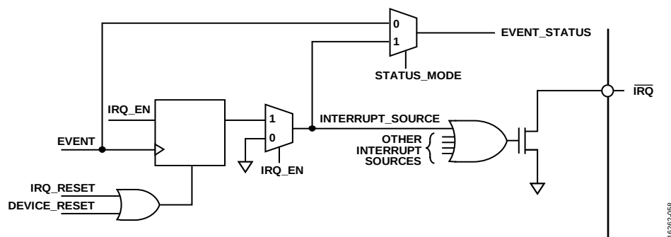
Figure 59. Simplified Schematic of \overline{IRQx} Circuitry
