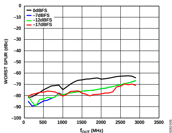
Figure 5. Worst Spur (dBc) vs. f_{OUT} over Digital Scale (Mode 0), 6 GHz DAC Sample Rate, Channel Interpolation 2 \times , Main Interpolation 8 \times
