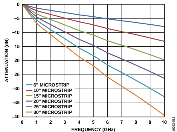
Figure 33. Insertion Loss of 50 \Omega Microstrips on FR4
