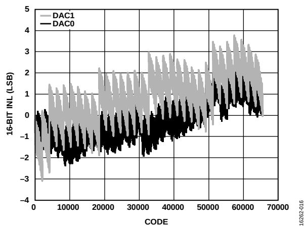
Figure 17. INL, I_{OUTFS} = 20 mA, 16-Bit Resolution
