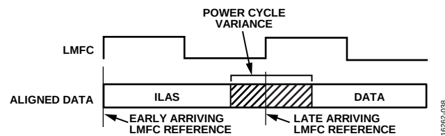
Figure 39. Link Delay &gt; LMFC Period Example
