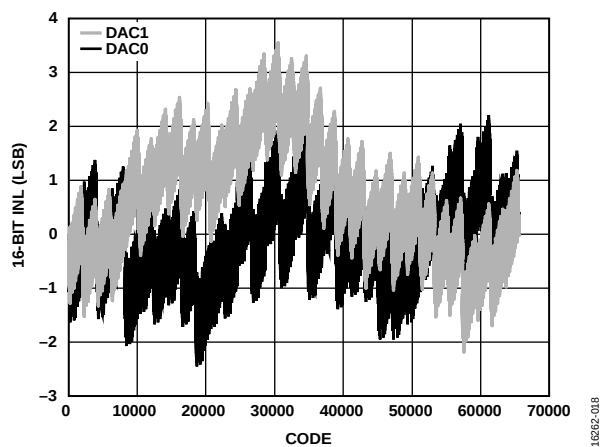
Figure 19. INL, I_{OUTFS} = 15.6 \text{ mA} , 16-Bit Resolution
