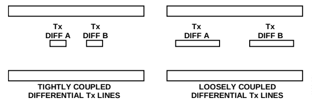
Figure 62. Tightly Coupled vs. Loosely Coupled Differential Traces
