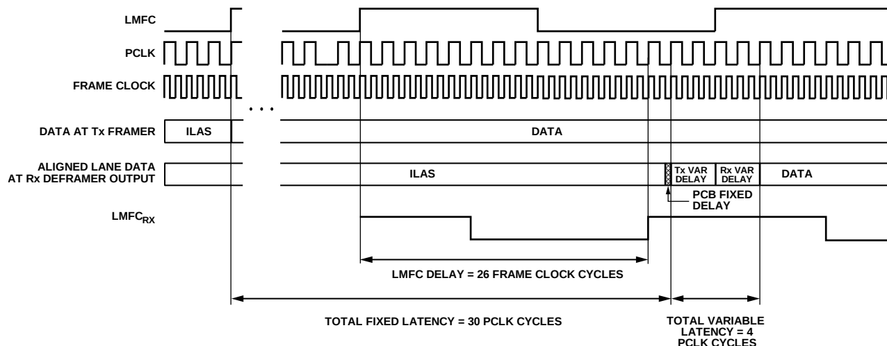
Figure 41. LMFC Delay Calculation Example
