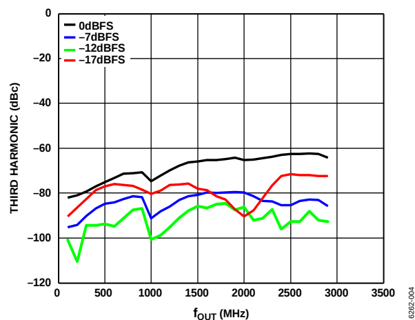
Figure 4. Third Harmonic (dBc) vs. f_{OUT} over Digital Scale (Mode 0), 6 GHz DAC Sample Rate, Channel Interpolation 2 \times , Main Interpolation 8 \times
