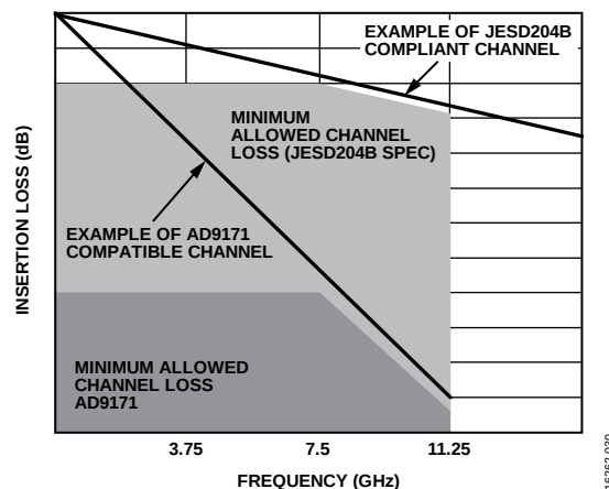
Figure 31. Insertion Loss Allowed
