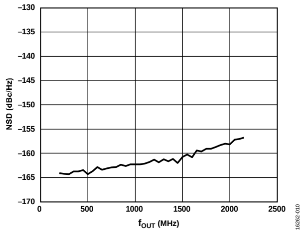
Figure 10. Single-Tone NSD Measured at 70 MHz vs. f_{OUT} , f_{DAC} = 5.89824 GHz, 12-Bit Resolution, Shuffle On
