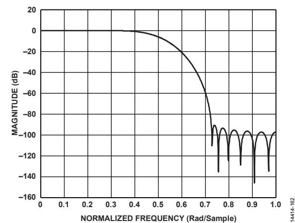
Figure 116. Second 2x Half-Band 45% Filter Response
