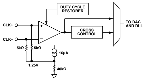
Figure 133. Clock Input
