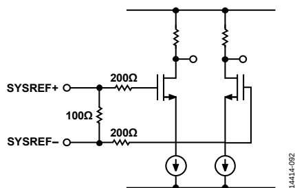
Figure 100. SYSREF± Input Circuit for the 8 mm × 8 mm 165-Ball BGA
