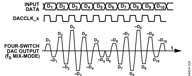
Figure 130. Mix-Mode Waveform
