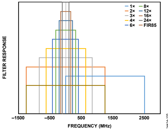
Figure 110. All Band Responses of Interpolation Filters
