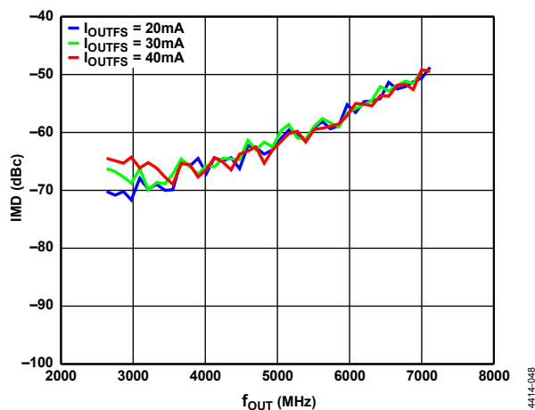
Figure 52. IMD vs. f_{OUT} over DAC I_{OUTFS}
