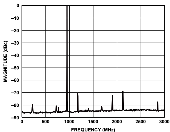
Figure 66. Single Carrier at 950 MHz Output
