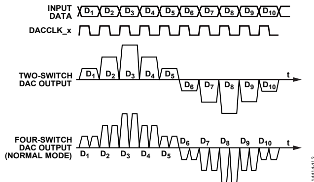
Figure 129. Two-Switch and Quad-Switch DAC Waveforms
