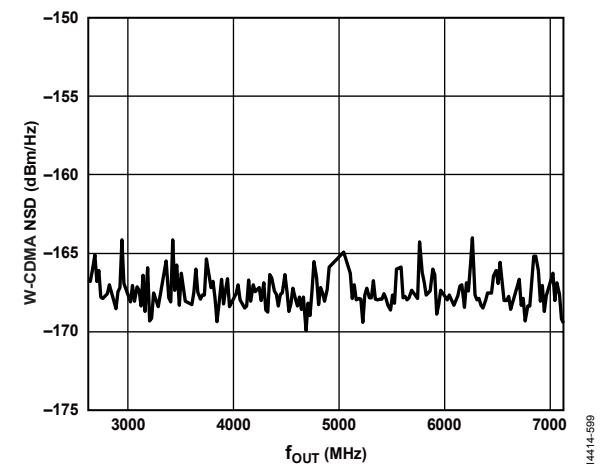
Figure 47. W-CDMA NSD vs. f_{OUT}
