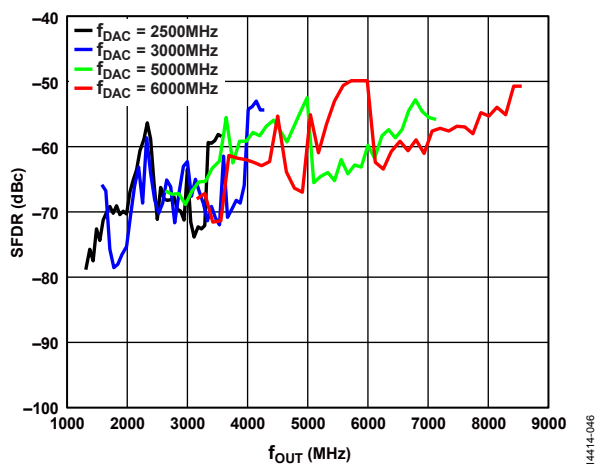
Figure 50. SFDR vs. f_{OUT} over f_{DAC}
