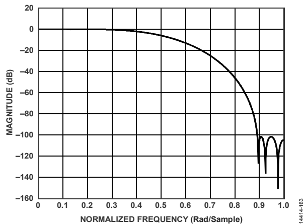
Figure 117. Third 2x Half-Band 22.5% Filter Response
