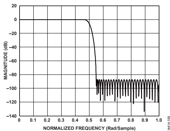
Figure 113. First 2x Half-Band 90% Filter Response
