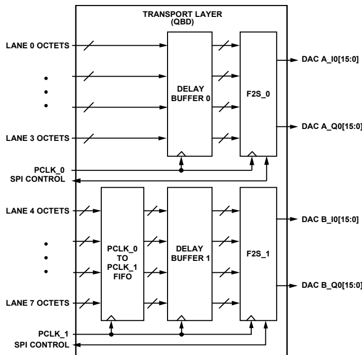
Figure 108. Transport Layer Block Diagram
