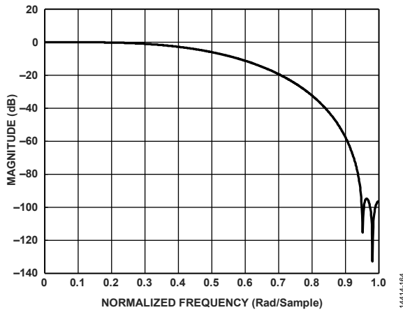
Figure 118. Fourth 2x Half-Band 11.25% Filter Response
