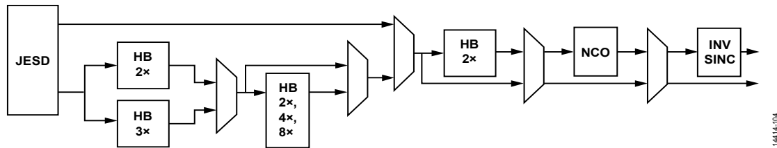
Figure 109. Block Diagram of the Main Digital Datapath
