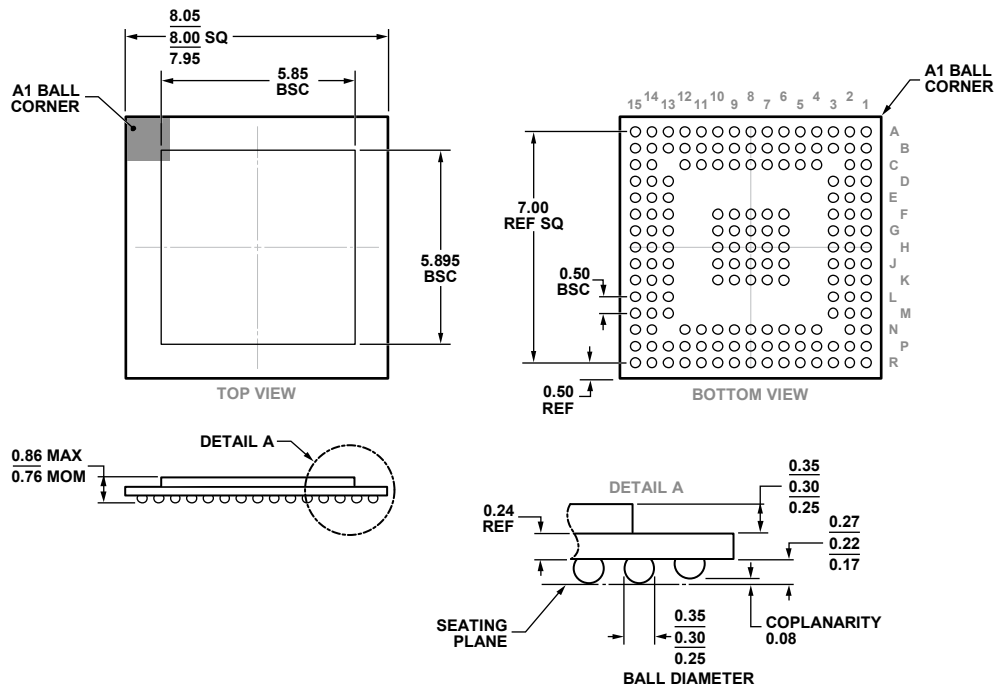
Figure 143. 165-Ball Chip Scale Package Ball Grid Array [CSP_BGA] (BC-165-1)
