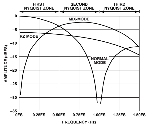
Figure 131. Sinc Roll-Off for NRZ, RZ, and Mix-Mode Operation
