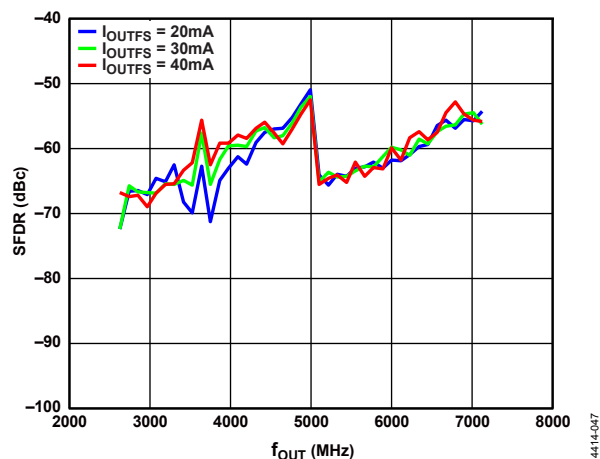
Figure 51. SFDR vs. f_{OUT} over DAC I_{OUTFS}
