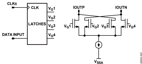
Figure 128. Quad-Switch Architecture
