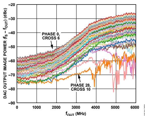
Figure 134. Performance Improvement from Tuning the Clock Input
