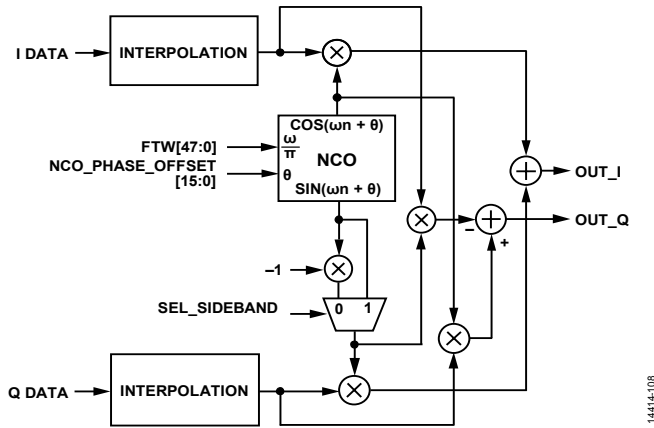
Figure 120. NCO Modulator Block Diagram
