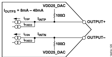
Figure 137. Equivalent DAC Output Circuit
