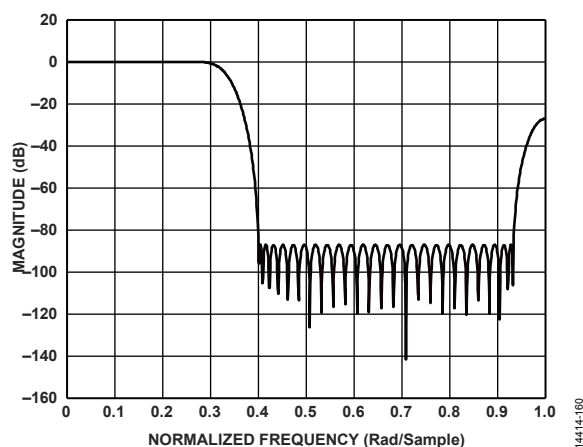
Figure 114. 3x Third-Band 80% Filter Response
