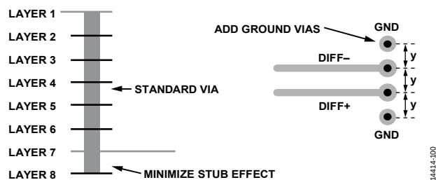
Figure 124. Minimizing Stub Effect and Adding Ground Vias for Differential Stripline Traces
