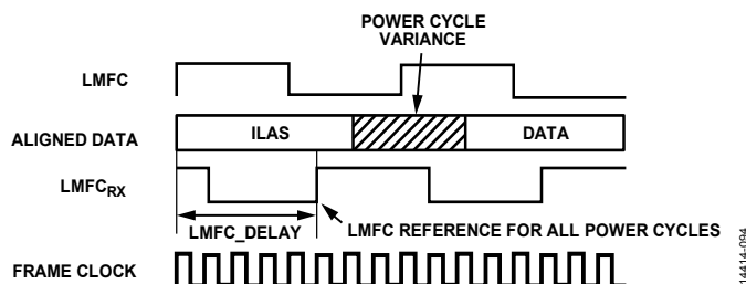
Figure 104. LMFC_DELAY_x to Compensate for Link Delay > LMFC
