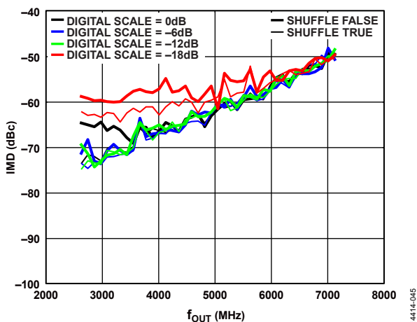
Figure 49. IMD vs. f_{OUT} over Digital Scale
