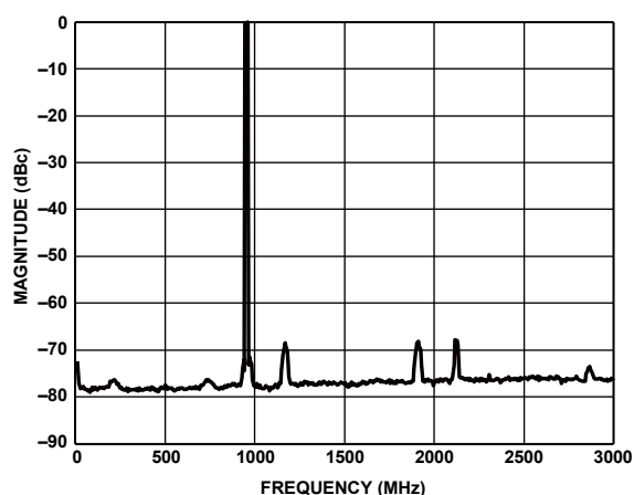
Figure 67. Four Carriers at 950 MHz Output
