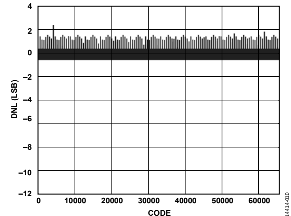
Figure 11. DNL, I_{OUTFS} = 40 mA
