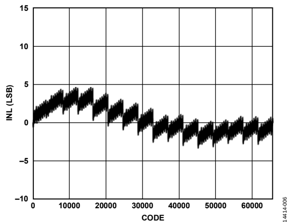
Figure 7. INL, I_{OUTFS} = 30 mA
