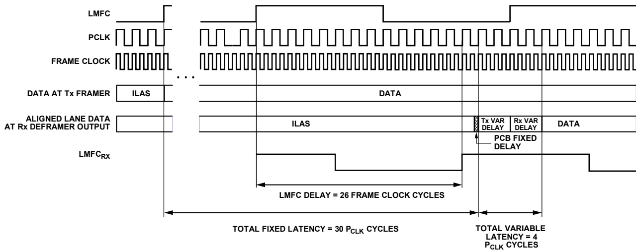
Figure 105. LMFC Delay Calculation Example
