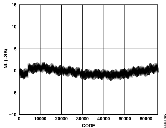
Figure 8. INL, I_{OUTFS} = 40 mA
