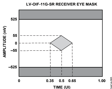
Figure 93. Receiver Eye Mask for 600 mV V TT Swing
