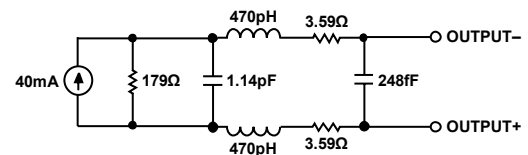
Figure 141. Equivalent Circuit Model of the DAC Output
