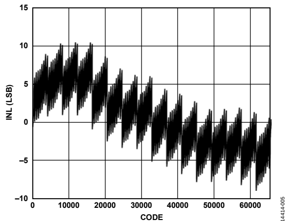
Figure 6. INL, I_{OUTFS} = 20 mA
