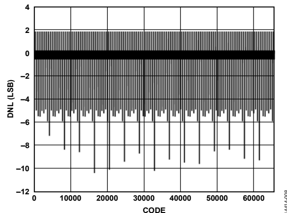
Figure 9. DNL, I_{OUTFS} = 20 mA
