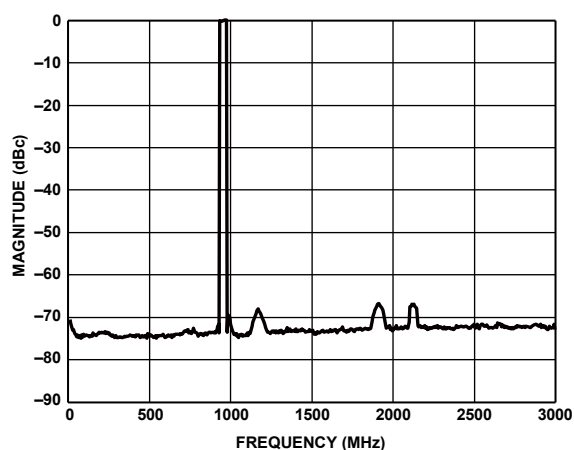
Figure 68. Eight Carriers at 950 MHz Output
