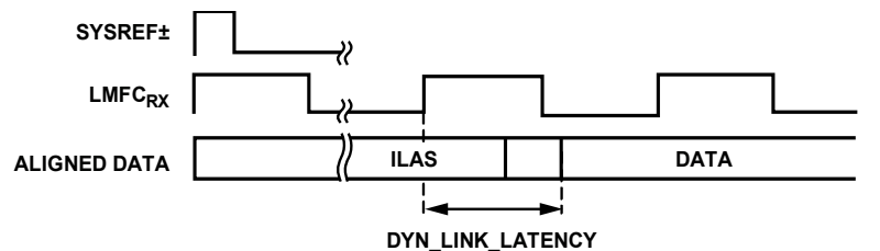
Figure 106. DYN_LINK_LATENCY_x Illustration
