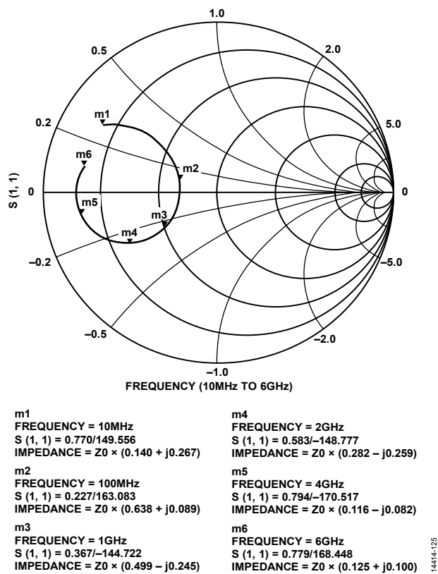
Figure 142. Simulated Smith Chart Showing the DAC Output Impedance Z_0 = 100 \Omega
