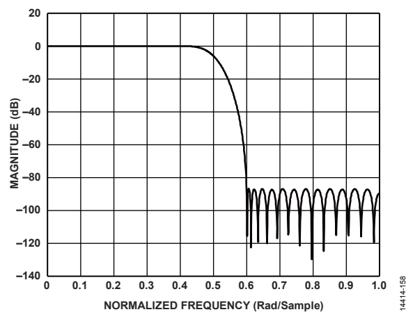
Figure 112. First 2x Half-Band 80% Filter Response
