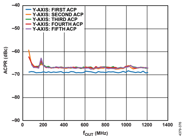
Figure 54. 16-Carrier ACPR vs. f_{OUT}
