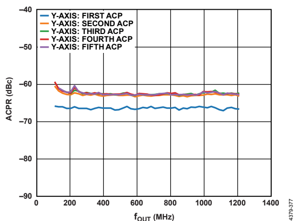
Figure 55. 32-Carrier ACPR vs. f_{OUT}
