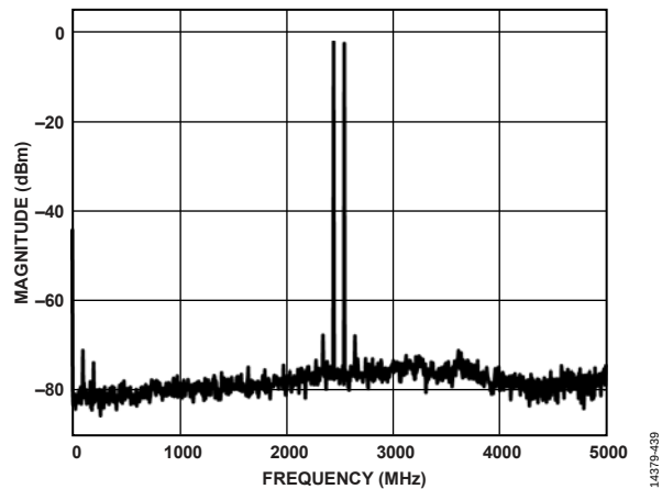
Figure 28. Single-Tone Spectrum at f_{OUT} = 2550\text{ MHz}
