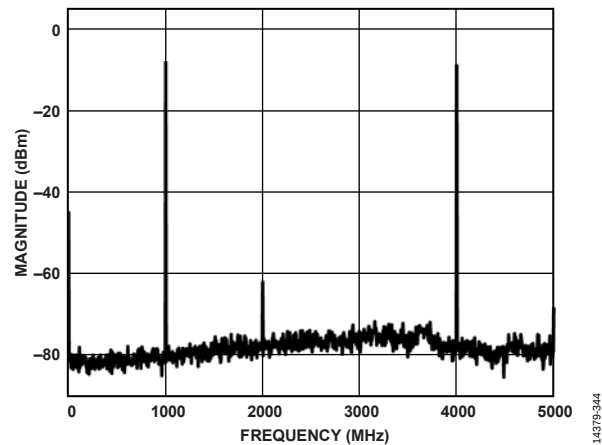
Figure 31. Single-Tone Spectrum at f_{OUT} = 4000\text{ MHz}
