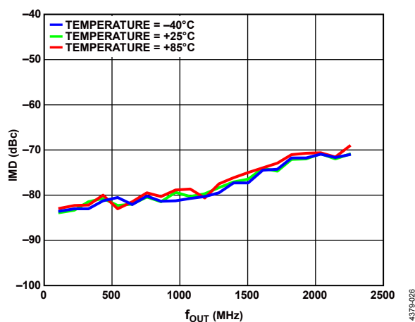
Figure 81. IMD vs. f_{OUT} over Temperature
